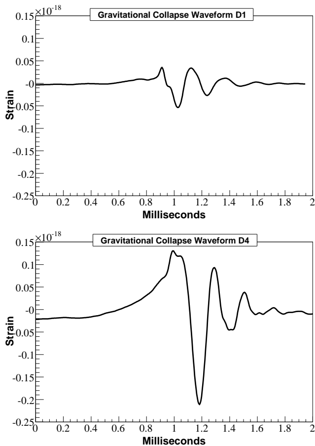
FIG. 4: Two example high frequency waveforms resulting from gravitational collapse of rotating neutron star models [9]. D1 results from a nearly spherical 1.26 solar mass star while D4 results from the collapse of a maximally deformed 1.86 solar mass star into a black hole. The figures show the plus polarization for each waveform (the cross polarization is at least an order of magnitude weaker in both cases) at a distance of 1 kpc, assuming optimal sky location and orientation. At this distance, the h_{\text{rss}} magnitudes of the two waveforms are 5.7 \times 10^{-22} \text{ Hz}^{-1/2} for D1 and 2.5 \times 10^{-21} \text{ Hz}^{-1/2} for D4. They differ from the figures presented in [9] in that the non-physical content at the beginning of the simulations has been removed.
