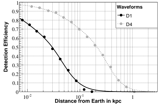
FIG. 6: Efficiency as a function of distance from Earth for supernova collapse waveforms D1 and D4 [9], assuming random sky location, polarization and inclination angle \iota . A \sin^2(\iota) dependence on the inclination angle was assumed.
