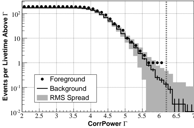
FIG. 9: CorrPower \Gamma distribution for background (normalized to the livetime of the analysis) and foreground distributions before the final CorrPower cut. The gray region is the RMS spread of counts in the background time-shifts while the error bars are the error in the mean counts per time-shift. The dotted line shows the cut at \Gamma=6.2 .
