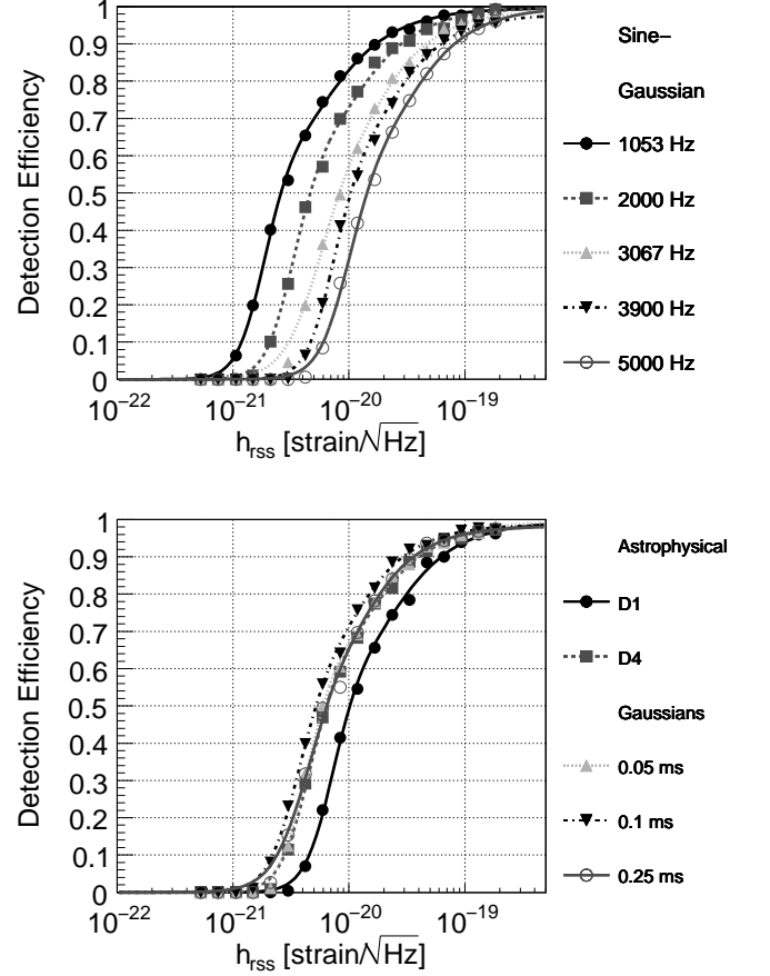
FIG. 5: Software injection efficiency curves for the set of sine-Gaussians of various frequencies (top) and Gaussians plus astrophysical waveforms (bottom). There is a consistent reduction in efficiency as a function of frequency following the noise distribution.
