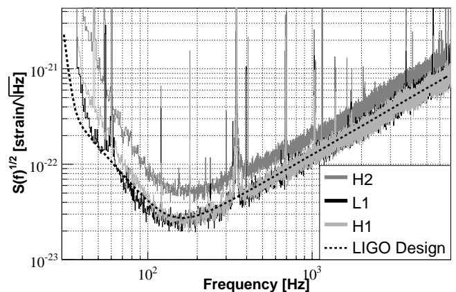
FIG. 1: Characteristic LIGO sensitivity curves from June 2006. Shot noise dominates the spectrum at high frequencies.
