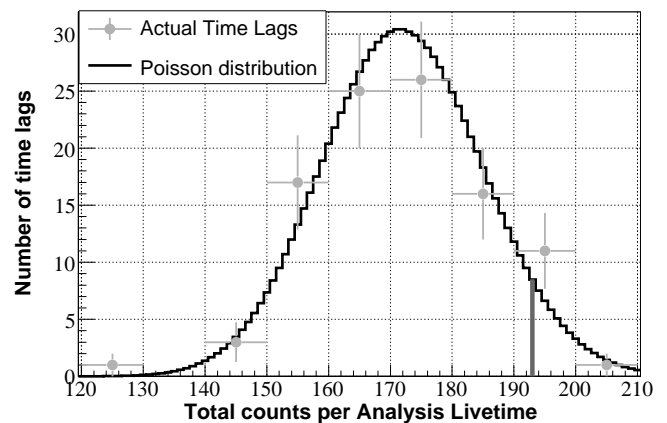
FIG. 8: Histogram showing number of time-shifts vs. counts normalized to analysis livetime. Superimposed is the expected distribution based on Poissonian statistics, which is consistent with the observed distribution. The black line at 193 counts indicates the actual number of foreground triggers observed.
