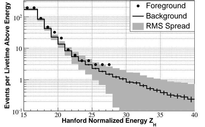
FIG. 10: QPipeline significance distribution for background (normalized to the livetime of the analysis) and foreground distributions at the Livingston (top) and Hanford (bottom) sites before the final CorrPower cut. The gray region is the RMS spread of counts in the background time-shifts while the error bars are the error in the mean counts per time-shift.
