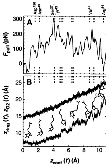
Fig. 3. (A) Pulling force exerted on the biotin molecule as a function of cantilever position z_{\text{cant}}(t) at a pulling velocity of 0.015 \text{ \AA ps}^{-1} (24). The dashed vertical lines mark the ruptures of hydrogen bonds (bold lines) and water bridges (thin lines) between the biotin and the indicated residues of the streptavidin binding pocket. (B) “Snapshot” of the motion of the biotin. The position of the oxygen atom O2 (see Fig. 1B) (upper curve), on which the pulling force was exerted, and the position of the center of mass of the ureido ring (lower curve), which points toward the interior of the binding pocket, are plotted as a function of cantilever position z_{\text{cant}}(t) . Eight “snapshots” of the biotin structure during rupture are depicted.
