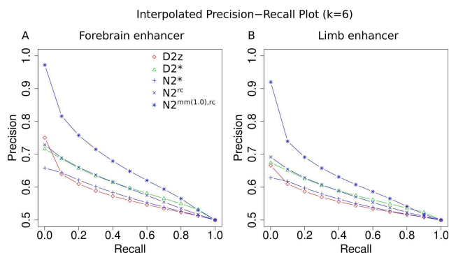
Fig. 3. Precision-Recall curve for enhancers active during mouse development. The plots show the precision average over 25 samples each time drawing 500 enhancer sequences ('positive') and 500 unrelated genomic sequences of equal length as the enhancers ('negative'). (A) Precision-Recall curve for forebrain enhancers. (B) Precision-Recall curve for limb enhancers.
