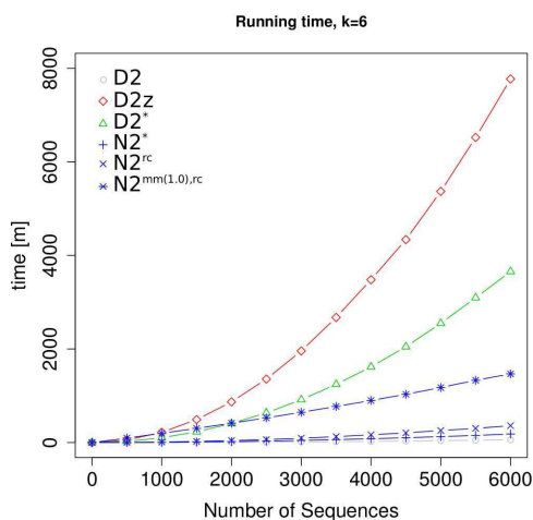
Fig. 1. Running time comparison. All pairwise scores were calculated for random sequences of length 1000bp.
