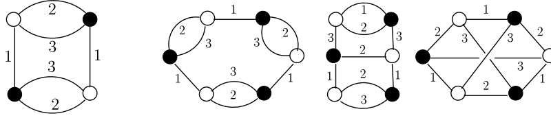
Figure 1. Some p -bubbles at p = 3 . Up to color relabeling, there is a single bubble with four vertices (on the left), whose invariant is \sum_{\{i_l, j_l\}} J_{i_1 i_2 i_3} \bar{J}_{i_1 j_2 j_3} J_{j_1 j_2 j_3} \bar{J}_{j_1 i_2 i_3} . But there exist different bubbles with six vertices (the three on the right).
