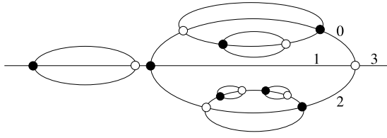
Figure 2. A patch of a melonic graph, recursively built by inserting on any line a pair of vertices, a black one and a white one, connected together via p lines (here p = 3 ).
