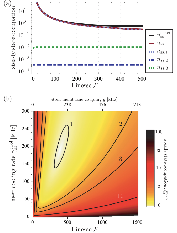
FIG. 4. (Color online) Sympathetic cooling of the membrane: Mechanical steady-state occupation number. (a) Approximate total occupation number n_{\text{ss}} with its individual contributions in the adiabatic limit [Eq. (38)] as a function of \mathcal{F} and for \gamma_{\text{at}}^{\text{cool}} = 240 kHz. For comparison, the exact mechanical occupation n_{\text{ss}}^{\text{exact}} , which results from solving the QLEs (31) and (35), is depicted as a black line. (b) Exact steady-state occupation number n_{\text{ss}}^{\text{exact}} as a function of \mathcal{F} and \gamma_{\text{at}}^{\text{cool}} . The top axis displays the corresponding coherent coupling g and the contours indicate the associated occupation numbers. For both plots the parameters from Table I have been used.
