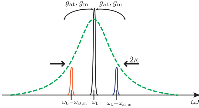
FIG. 2. (Color online) Light fields involved in mediating the effective coupling. The laser-enhanced interactions (coupling constants g_m and g_{at} ) correspond to a conversion between laser photons \omega_L (black) and sideband photons \omega_L \pm \omega_{at,m} [blue (dark) and red (light)]. The response profile of the cavity is indicated by the green dashed line and easily accommodates both sidebands in the bad cavity regime discussed in the text.
