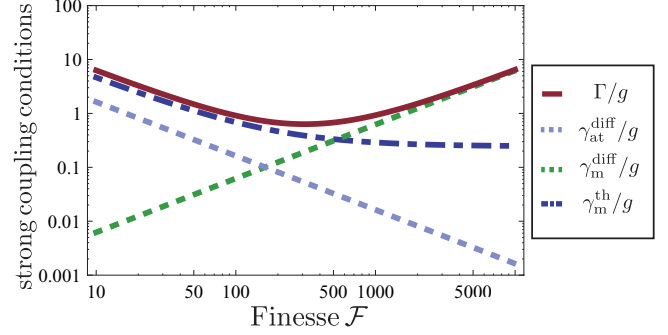
FIG. 3. (Color online) Coherent dynamics: We plot the ratios \gamma_{\text{at}}^{\text{diff}}/g , \gamma_m^{\text{diff}}/g , and \gamma_m^{\text{th}}/g as a function of finesse to illustrate the strong-coupling conditions in Eq. (34). One clearly observes a tradeoff between mechanical heating ( \gamma_m^{\text{th}} ) and radiation pressure noise ( \gamma_m^{\text{diff}} ). Parameters other than \mathcal{F} are taken from Table I.
