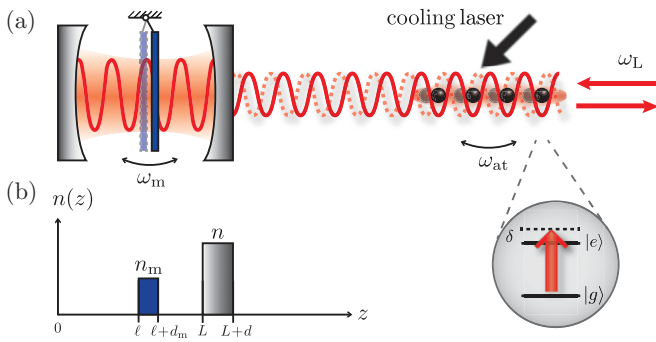
FIG. 1. (Color online) (a) Micromechanical membrane in a cavity coupled to a distant atomic ensemble by means of a laser (red, frequency \omega_L ). The motion of the membrane shifts the optical lattice dipole trap of the atoms, while the motion of the atoms changes the radiation pressure on the membrane. Inset: The atoms are modeled as two-level systems, which are far off resonant with respect to the laser. (b) Refractive index profile used in the one-dimensional model [Eq. (6)].
