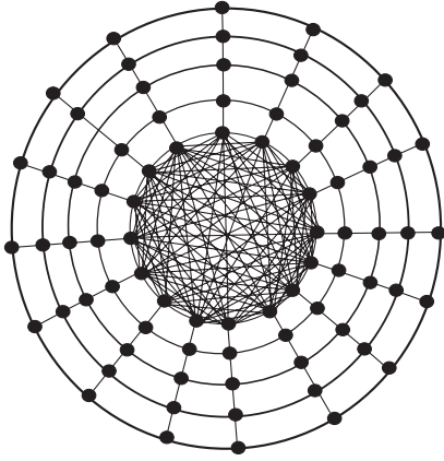
FIG. 7. The \mathcal{K}_N graph.
