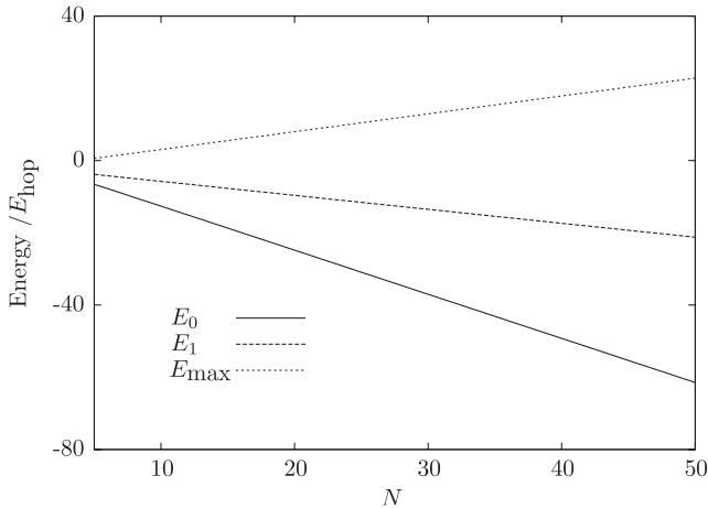
FIG. 10. Plot of the energies of the ground state E_0 , the first excited state E_1 , and the state with maximum energy E_{\text{max}} , with respect to the size of the trapping surface, N , for a rotational invariant graph with decaying connectivity (1 + N/r) , in the single particle sector. Note that the gap E_1 - E_0 increases linearly with N .
