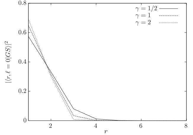
FIG. 11. Probability distribution of the position of the particle. The particle is completely confined around the trapping surface. The larger the falloff coefficient \gamma , the larger the confinement.
