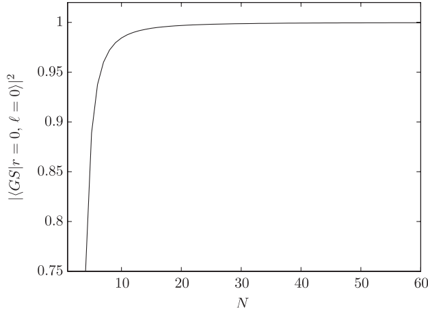
FIG. 9. Fidelity between the completely delocalized state in the completely connected region |r = 0, \ell = 0\rangle and the ground state against the size N of that region. The completely delocalized state |r = 0, \ell = 0\rangle becomes the ground state of the system for large N .
