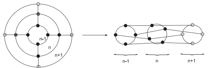
FIG. 3. A 2-d lattice that can be foliated.
