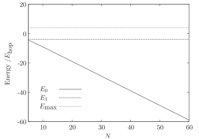
FIG. 8. Plots of the energy E_0 of the ground state, the energy E_1 of the first excited state, and E_{\text{max}} , the energy of the maximum energy state, against the size N of the completely connected region of the \mathcal{K}_N graph, in the single particle sector. This plot has been realized for the full model with R = 30 . Note that the gap E_1 - E_0 increases linearly with N .
