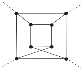
FIG. 5. A foliated graph which is not rotationally invariant.
