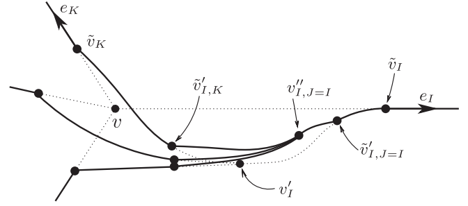
FIG. 3. Sample deformation produced by two successive singular diffeomorphisms along the edge e_I . Here the dotted lines indicate the position of the graph before the deformations; these are not part of the resulting graph. The structure of the deformations is similar to that produced by the action of two successive Hamiltonian-type deformations, except that now the original vertices v and v'_I are charged in no copies of U(1) ; the dotted edges are not actually there. Note that the kink structure is the same as for the Hamiltonian deformations: the edge e_I is C^1 at \tilde{v}_I and \tilde{v}'_{I,J=I} , but all other edges are C^0 at the various \tilde{v}_K and \tilde{v}'_{I,K} .
