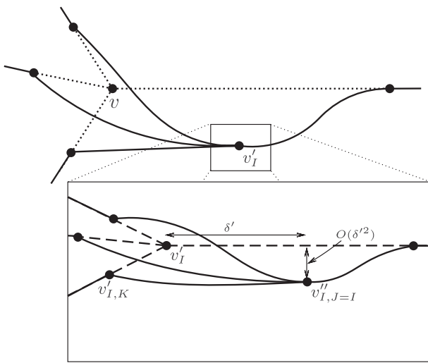
FIG. 2. Detail of the deformation generated by two successive Hamiltonian actions, in this case along the same edge J = I . Here \delta' \ll \delta .
