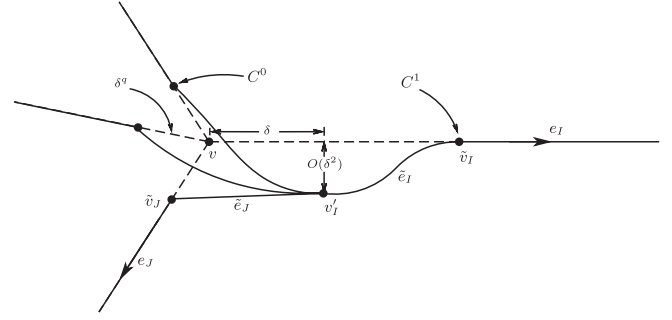
FIG. 1. A sample deformation produced by a single Hamiltonian constraint action at a nondegenerate vertex v along the edge e_I . The dashed edges emanating from the original vertex v are now only charged in two of the three U(1) factors, but v_I^a is expected to be, generically, nondegenerate. With respect to the coordinate system fixed at v , v_I^a is located a distance \delta from v along \dot{e}_I and displaced off of e_I a distance O(\delta^2) . \tilde{e}_I and e_I share a tangent at \tilde{v}_I , but \tilde{e}_J and e_J do not share a tangent. All of the \tilde{e}_{J \neq I} have tangents at v_I^a which are bunched and lie within a cone of apex angle O(\delta^{q-1}) .
