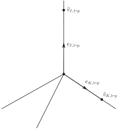
FIG. 5. The 1-past \gamma_{1-p}(c) .
