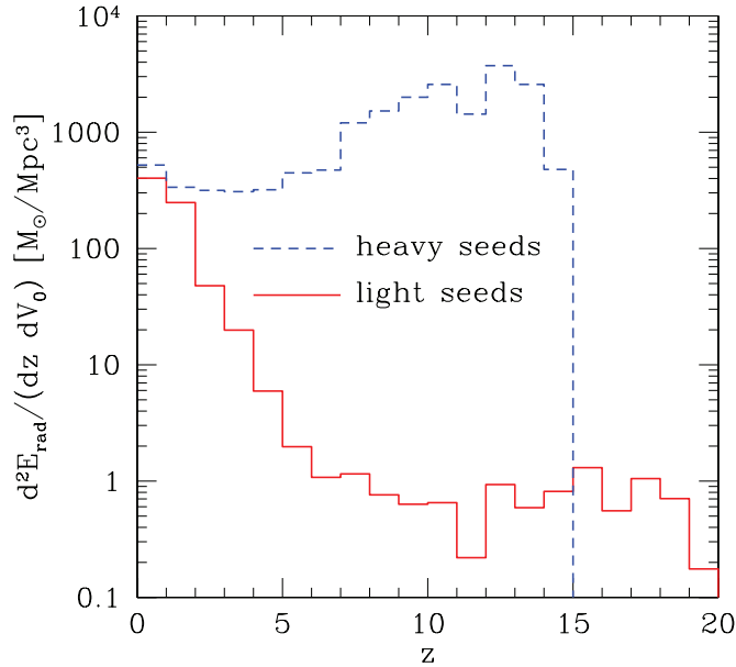
Figure 4. Energy emitted by massive BH mergers per unit redshift and unit comoving volume, as a function of redshift. The two lines refer either to the “light-seed” scenario (red solid curve) or to the “heavy-seed” scenario (blue dashed line).
