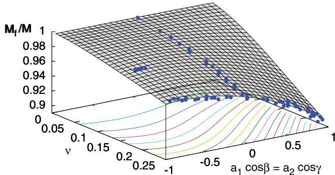
Figure 3. Mass of the final BH, M_f \equiv M - E_{\text{rad}} , and corresponding fit for all the published binaries with a_1 \cos \beta = a_2 \cos \gamma . Note the simple functional dependence of the E_{\text{rad}} , whose behavior can be well captured with low-order polynomials.
