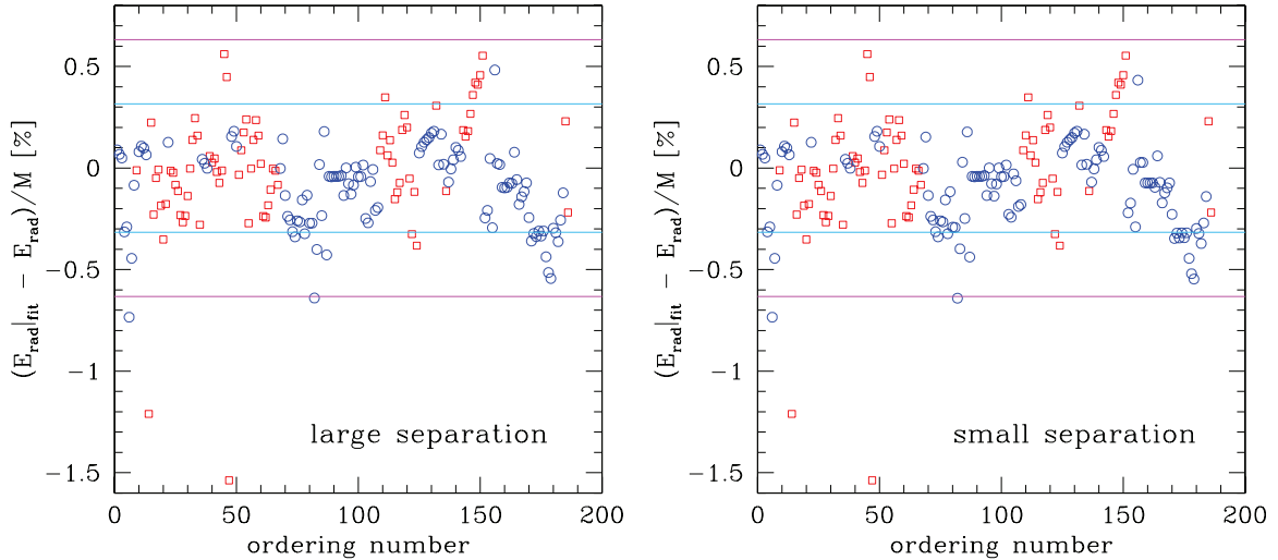
Figure 2. Residuals for the fitting formula at small and large separations as a function of a dummy index representing the binaries in our data set. Binaries with spins aligned/antialigned with the orbital angular momentum are plotted in red/boxes, while binaries with misaligned spins are shown in blue/circles. Cyan and violet lines represent the 1\sigma and 2\sigma errors (estimated a posteriori) of the data with spins aligned/antialigned with the orbital angular momentum. The first 50 points correspond to the simulations performed after 2010.
