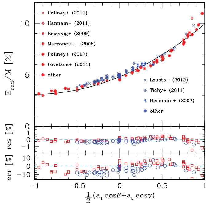
Figure 1. Top panel: radiated energy, E_{\text{rad}}/M , as a function of the total spin of the system along the orbital angular momentum, |a_1| \cos \beta + |a_2| \cos \gamma , for all published NR simulations with q = 1 , both with aligned/antialigned spins (in red/boxes) and for misaligned spins (in blue/circles). Shown instead with a black solid line is the prediction of expression (14) with the coefficients fitted from aligned/antialigned binaries. Bottom panels: residuals of the NR data from the fitting expression and the corresponding error relative to E_{\text{rad}}/M . (A color version of this figure is available in the online journal.)
