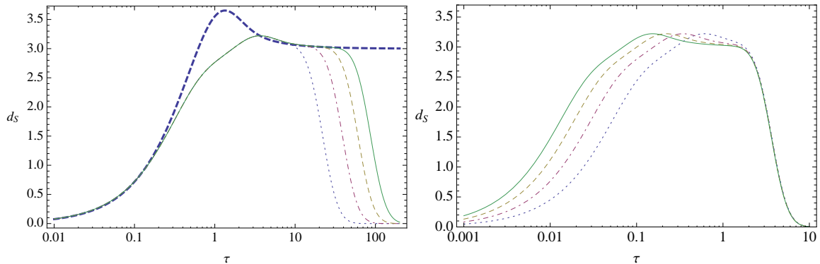
Figure 7. Left: (a) equilateral T^3 triangulation in terms of N_0 = p^3 vertices, p = 6, 8, 10, 12 from left to right (dotted, dot-dashed, dashed thin, solid curve), compared with the cubic lattice (dashed thick). Right: (b) rescaled triangulations.
