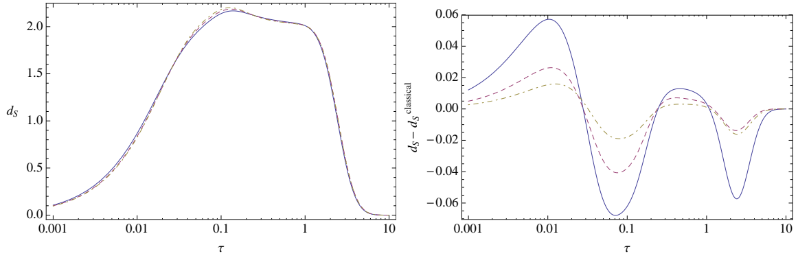
Figure 11. Left: d_S for coherent states peaked at l(J) = J + 1/2 = 16, 32, 64 (solid, dashed and dot-dashed curve) on a regular torus triangulation (with N_2 = 18 \times 4^2 = 288 triangles) with spread \sigma = \sqrt{J-1/2} . Right: deviation of d_S from the classical case.
