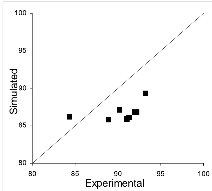
Figure 16. Experimental and simulated conversion of isobutene (all 11 test runs) for the column with the reactive section filled with catalytic structured packing Montz Multipak.
