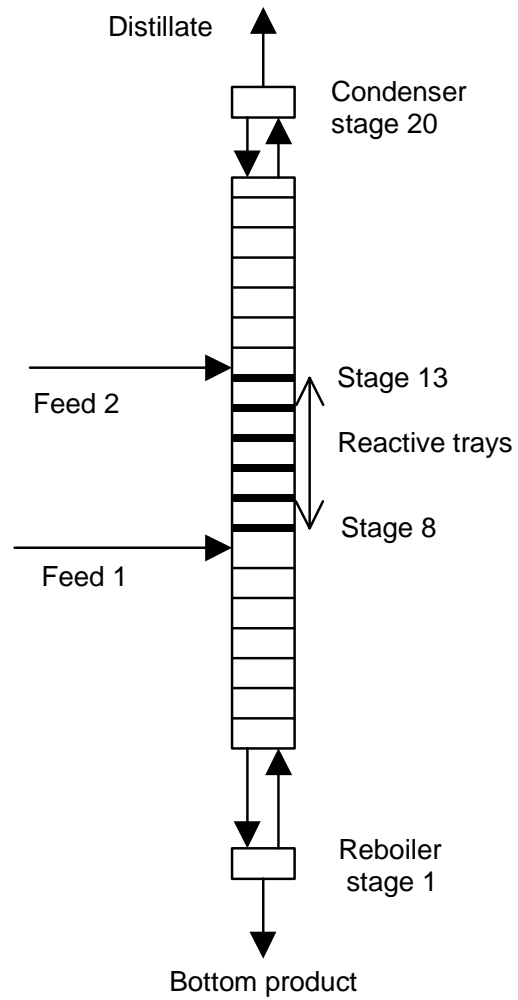
Figure 6. Scheme of the column used in examples for the eddy diffusion model and mixed pool model.
