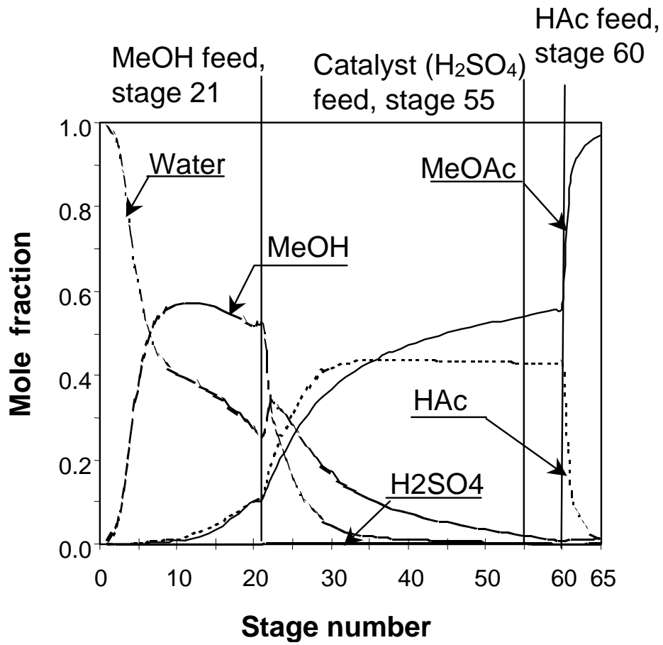
Figure 15. Simulation of methyl acetate synthesis, liquid composition profiles.
