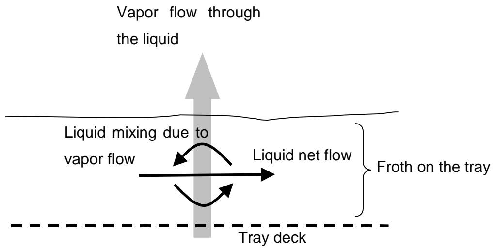
Figure 2. The eddy diffusion model of a distillation tray.
