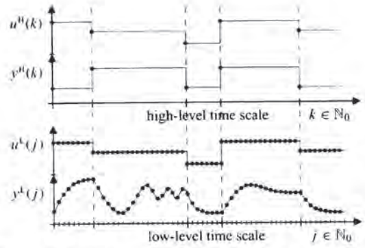
Fig. 2. Relation between time scales in \mathfrak{B}_{\text{im}}
