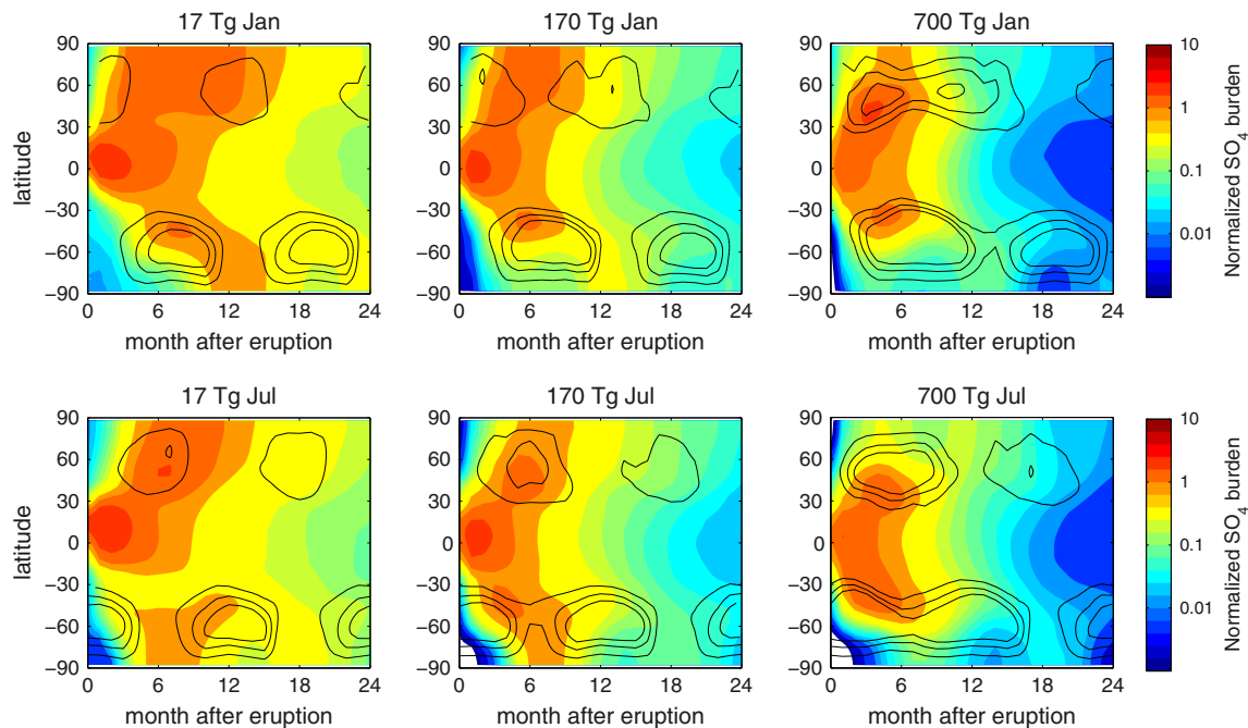
Figure 5. Normalized zonal mean sulfate aerosol burden as a function of month after eruption for January (top) and July (bottom) eruptions, for 17, 170, and 700 Tg \text{SO}_2 injection experiments (left to right). Also shown are zonal mean zonal westerly winds in the lower stratosphere (50 hPa), with contours at 10, 20, and 30 m/s.
