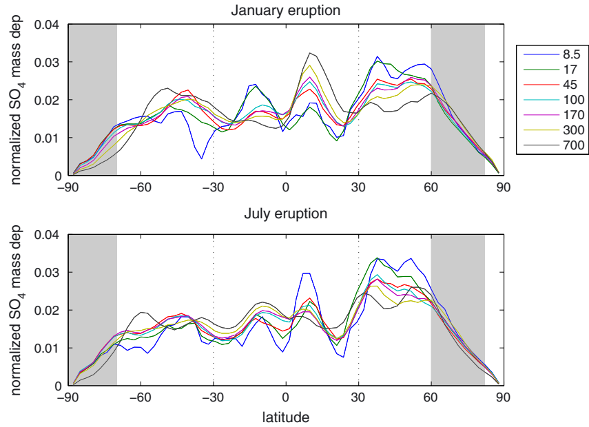
Figure 4. Normalized zonal sulfate mass deposition for tropical stratospheric \text{SO}_2 injections of varying magnitudes as indicated in legend (in Tg). The deposition distributions are normalized by dividing the sulfate mass deposited in each latitudinal band by the total global mass deposition. Gray shading indicates the approximate latitude ranges of Antarctica ( 70^\circ\text{S} – 90^\circ\text{S} ) and Greenland ( 60^\circ\text{N} – 80^\circ\text{N} ).
