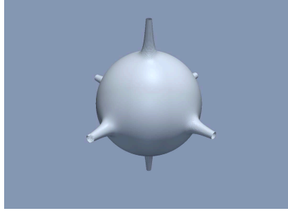
Fig. 1 A two-dimensional section of the N = 8 S^3 black-hole lattice, embedded in three dimensions.
