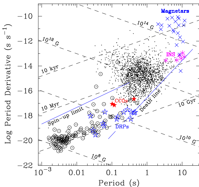
FIG. 1.— Pulsar populations on the P - \dot{P} diagram, including magnetars (blue crosses), INs (magenta asterisks), CCOs (filled red stars) and DRPs (open blue stars). Black dots are isolated pulsars and circled dots are pulsars in binaries. (Pulsars in globular clusters are excluded as their period derivatives are not entirely intrinsic.) Dashed lines of constant characteristic age and magnetic field are indicated.
