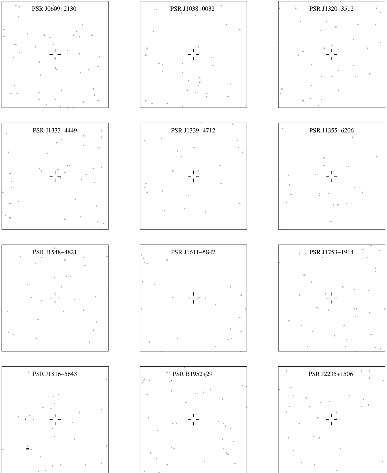
FIG. 2.— Chandra ACIS-S 0.3 – 10 keV X-ray images of targeted radio pulsars listed in Table 1. Each grey square is a detected count and black squares contain two counts. A nearby source to PSR J1816-5643 is evident by a cluster of counts. No X-ray sources are found within the adopted 1''.2 radius Chandra error circle centered on the radio coordinates (crosses). The plots are 45'' on a side; the inner dimensions of the crosses are 2'' .
