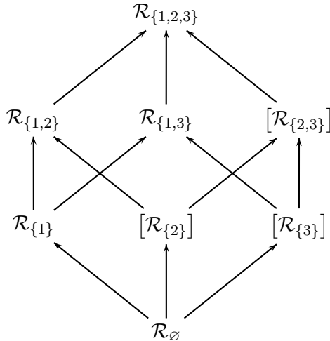
Figure 1: Hasse diagram for the unitary highest weight representations of \mathfrak{u}(1,2) algebra. The brackets [ \ ] indicate that the enclosed Lax operator has non-polynomial matrix elements. If the bracket is absent, one may normalize the Lax operator such that its matrix elements are polynomial.
