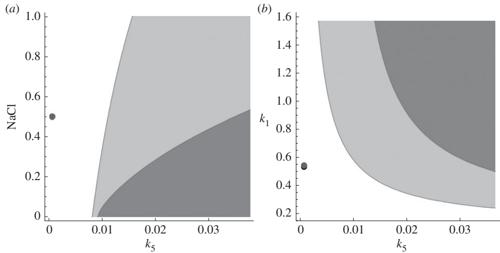
Figure 6. Stability region plots for the HOG system. ( a,b ) Shows stability regions for different parameter combinations. In ( a,b ), dark grey and light grey indicate regions with unstable steady state, i.e. where oscillations occur, for the system with (model no. 6) and without autoinhibitory feedback (model no. 2), respectively. Black and dark grey dots indicate the fitted parameters for the system with (model no. 6) and without autoinhibitory feedback (model no. 2), respectively. The boundary between white and shaded regions indicates bifurcation lines in the respective two-dimensional parameter space. For more stability region plots for different parameter combinations, please refer to the electronic supplementary material.
