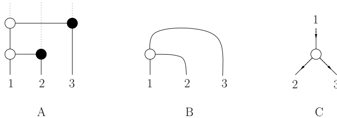
Fig. 3 Three-point \overline{\text{MHV}} Yangian invariant. A) Transposition decomposition; B) wilted on-shell diagram; C) on-shell diagram with a perfect orientation.
