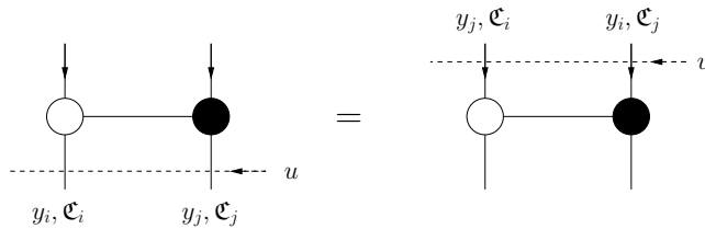
Fig. 1 Fundamental relation (48) for the construction of Yangian invariants using the intertwining operators \mathcal{B}_{ij}(y_i - y_j) .
