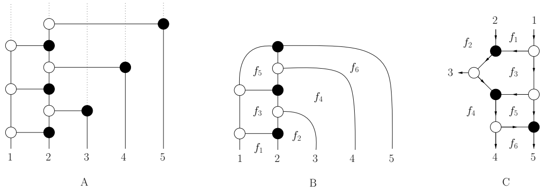
Fig. 6 Five-point MHV Yangian invariant. A) Transposition decomposition; B) wilted on-shell diagram; C) on-shell diagram with a perfect orientation.
