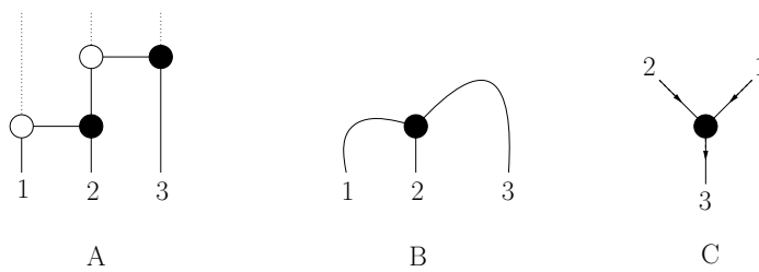
Fig. 4 Three-point MHV Yangian invariant. A) Transposition decomposition; B) wilted on-shell diagram; C) on-shell diagram with a perfect orientation.
