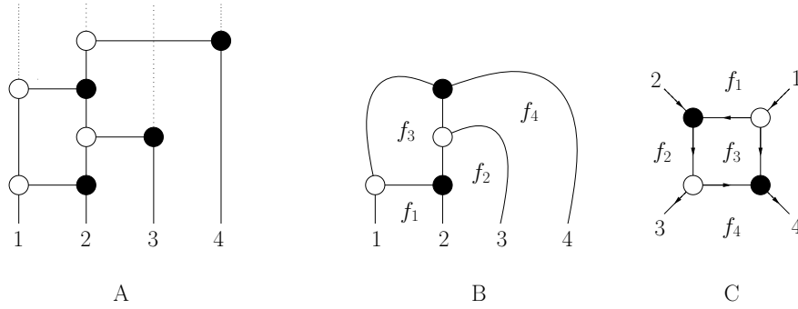
Fig. 5 Four-point MHV Yangian invariant. A) Transposition decomposition; B) wilted on-shell diagram; C) on-shell diagram with a perfect orientation.
