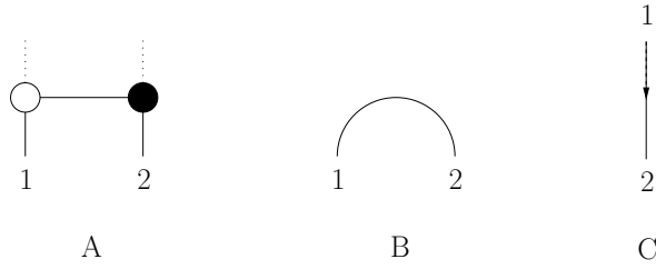
Fig. 2 Two-point Yangian invariant. A) Transposition decomposition; B) wilted on-shell diagram; C) on-shell diagram with a perfect orientation.
