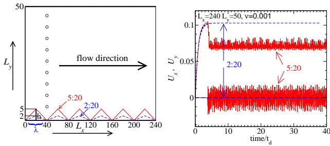
Figure 2: Left: A sketch of the simulation box for two choices of the wall roughness. The top wall is assumed to be flat, whereas the bottom wall has a zig-zag form. A zig-zag wall can be characterized by two numbers: The height, h , of the roughness tip and the half-wave length \lambda/2 . We use the notation h : \lambda/2 for a given zig-zag wall. Flow velocity versus time is recorded at equidistant points along the line x = 40 (open circles). Note that the region below the zig-zag line is filled with solid particles (not shown for clarity). Right: Parallel, U_x , and the perpendicular, U_y , components of the fluid velocity in the middle of the flow region versus time for both choices of the wall roughness shown in the left panel. The time axis is rescaled by the momentum diffusion time. Note the strong fluctuations of the vertical component of the velocity in the case of the 5:20 zig-zag surface.
