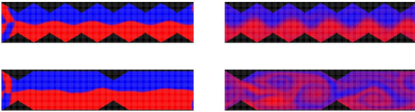
Figure 5: Impact of the channel design on mixing. In a zig-zag channel (top), 2/3 of all teeth are removed (bottom). A flow which is not that irregular (top) then becomes fully chaotic (bottom) leading to an efficient mixing. Left: initial stage. Right: after a time of 10^{-2} \times t_{\text{diff}} , where t_{\text{diff}} is the time necessary for diffusion to achieve complete mixing.
