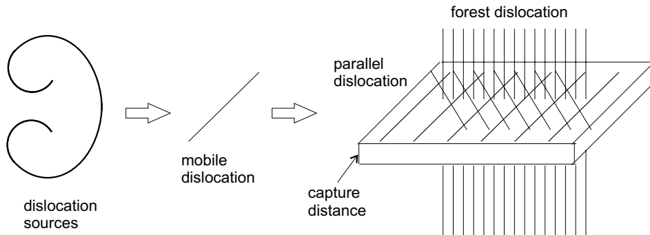
Fig. 1. Schematic drawing of the slip mechanism for the fcc crystal structure: a mobile dislocation is generated by a frank-read source, in order to move it must overcome the resistances of forest and parallel dislocations with the help of the external stress.
