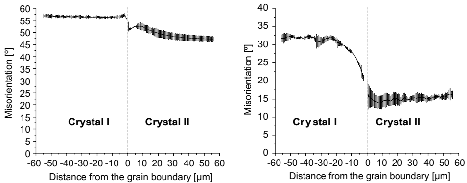
Fig. 7. Average misorientation relative to the initial orientation measured for the two bicrystals.
