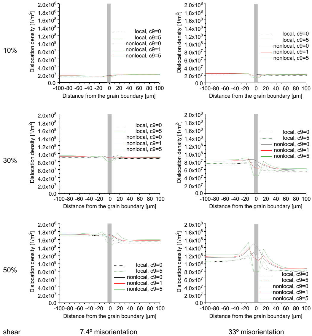
Fig. 12. Statistically stored dislocation density calculated for the two bicrystals for simulation cases (1)–(5). The range of the grain boundary element is indicated by the grey bar.
