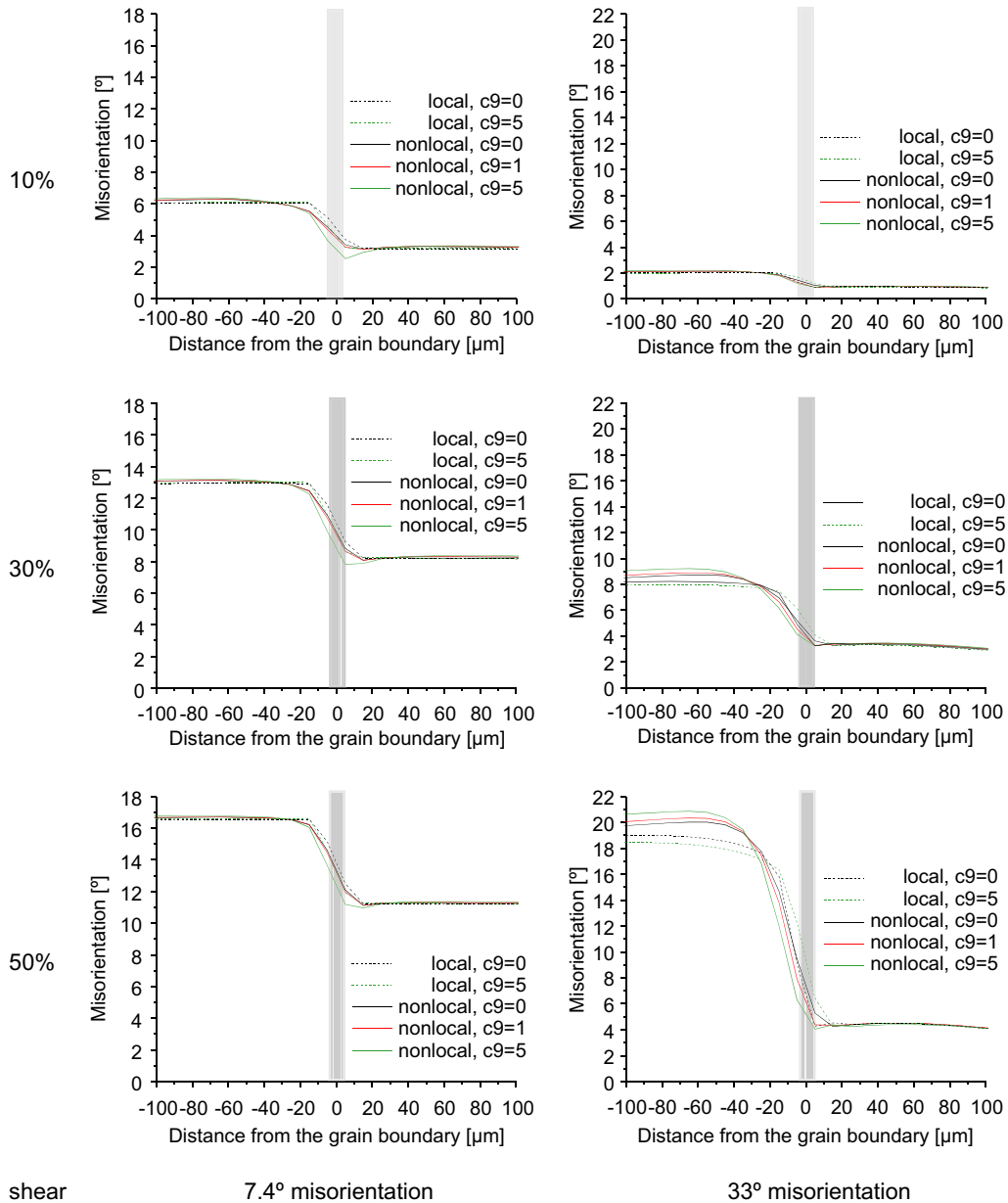
Fig. 8. Misorientation calculated for the two bicrystals for simulation cases (1)–(5). The range of the grain boundary element is indicated by the grey bar.
