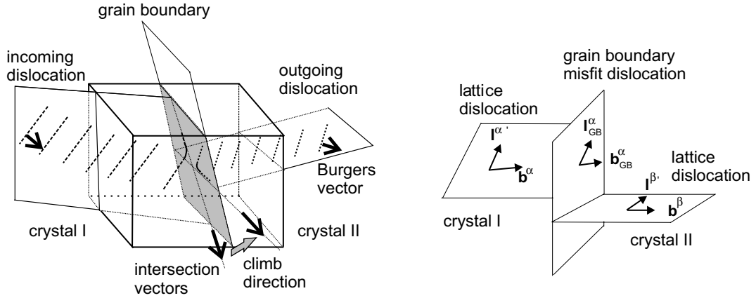
Fig. 2. Schematic drawing of a penetration event from crystal I to crystal II.
