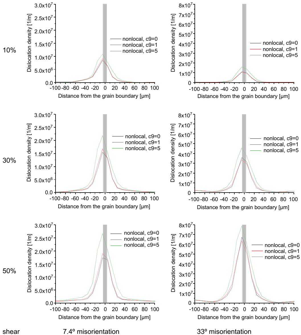
Fig. 13. Geometrically necessary dislocation density calculated for the two bicrystals for simulation cases (1)–(5). The range of the grain boundary element is indicated by the grey bar.
