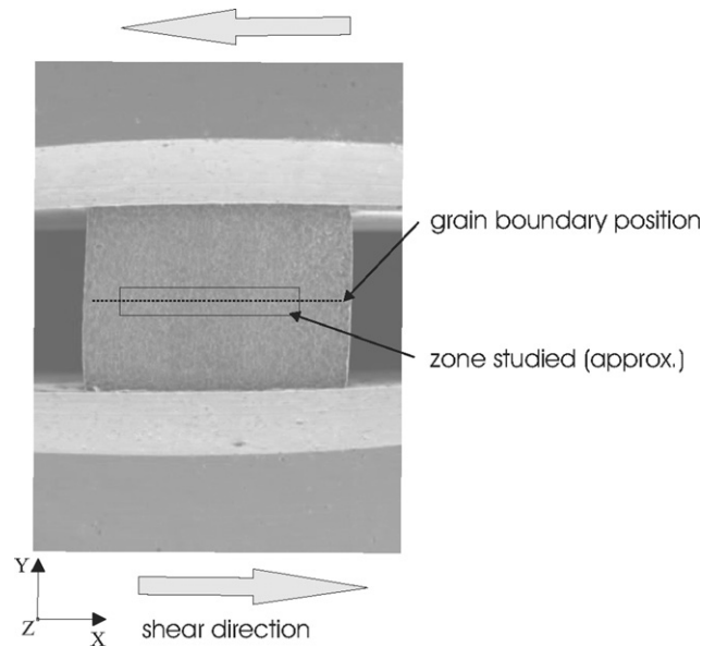
Fig. 5. Experimental set-up and the position of the studied zone across the grain boundary.
