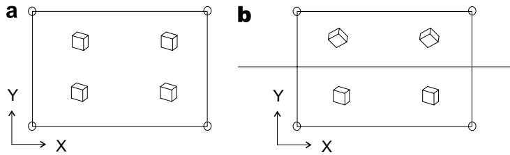
Fig. 3. 2D schematic drawing of a bulk element (a) and a grain boundary element (b) in their initial state. During the deformation GNDs should preserve the continuity of lattice in X - and Y -direction for bulk elements, while for grain boundary elements only the X -direction is considered.
