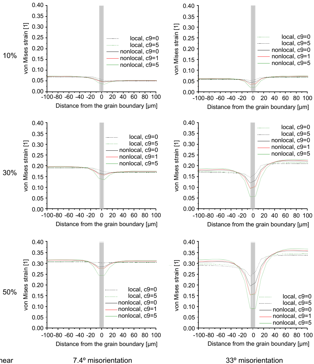
Fig. 11. von Mises strain calculated for the two bicrystals for simulation cases (1)–(5). The range of the grain boundary element is indicated by the grey bar.
