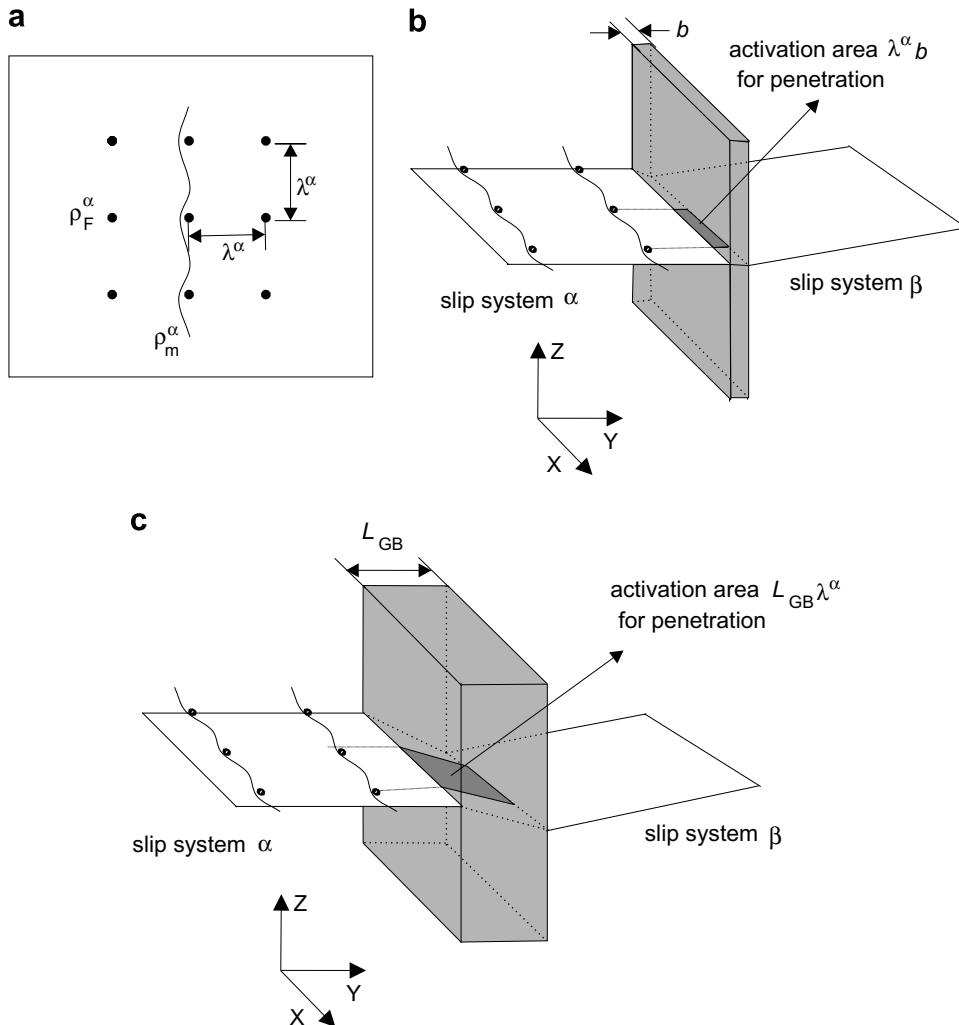
Fig. 4. Schematic drawing of the penetration and cutting mechanism: (a) cutting mechanism; (b) penetration of perfect grain boundary; (c) FEM treatment of penetration process.
