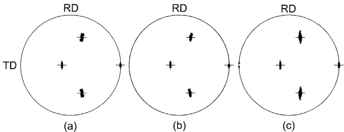
Fig. 3. (111) pole figures calculated by FEM for (112)[1\bar{1}0] initial center orientation with (a) (001)[1\bar{1}0] , (b) (41342)[13\bar{4}0] and (c) (110)[1\bar{1}0] surrounding orientations.
