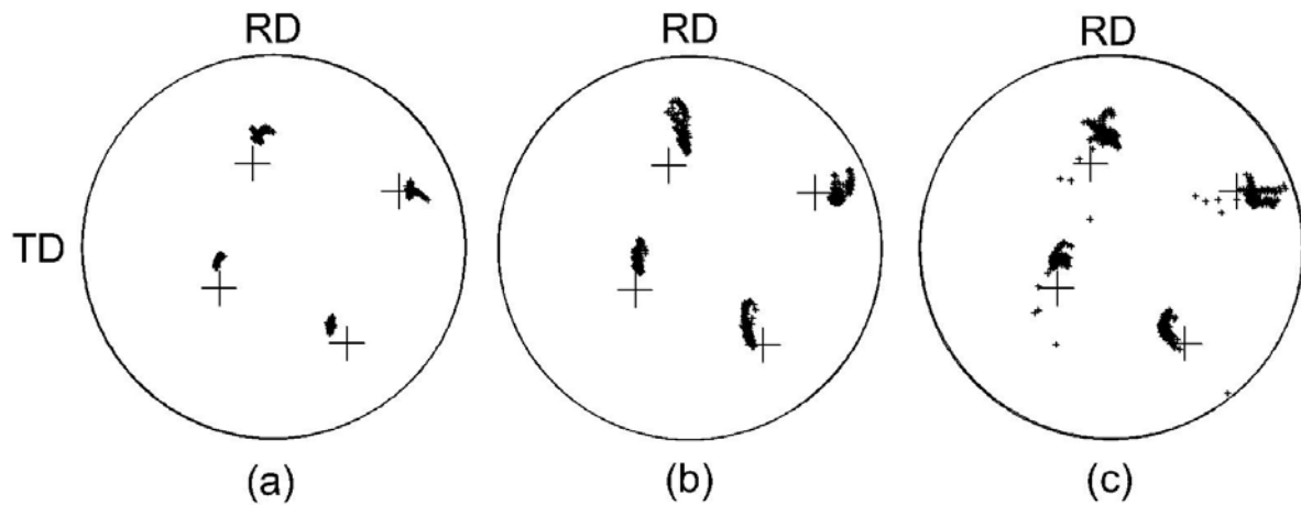
Fig. 4. (111) pole figures calculated by FEM for (13\ 4\ 42) [4\ \bar{13}\ 0] initial center orientation with (a) (0\ 0\ 1) [1\ \bar{1}\ 0] , (b) (4\ 13\ 42) [13\ \bar{4}\ 0] and (c) (1\ 1\ 0) [1\ \bar{1}\ 0] surrounding orientations.
