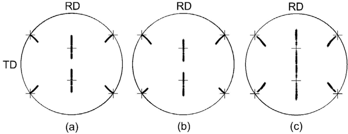
Fig. 5. (111) pole figures calculated by FEM for (011)[100] initial center orientation with (a) (001)[1\bar{1}0] , (b) (41342)[13\bar{4}0] and (c) (110)[1\bar{1}0] surrounding orientations.
