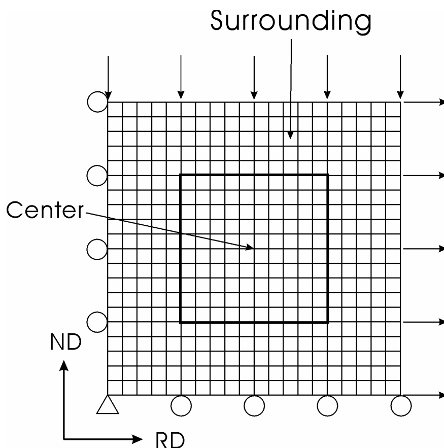
Fig. 1. Initial finite element mesh.
