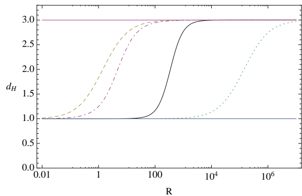
FIG. 6. Hausdorff dimension d_{\text{H}} of a superposition with \alpha = 1, 2 (solid and dash-dotted curve) in d = 3 summing up to j_{\max} = 10^5 , compared to d_{\text{H}} on single states |1, \mathcal{C}_\infty\rangle (dashed curve) and |j_{\max}, \mathcal{C}_\infty\rangle (dotted curve).
