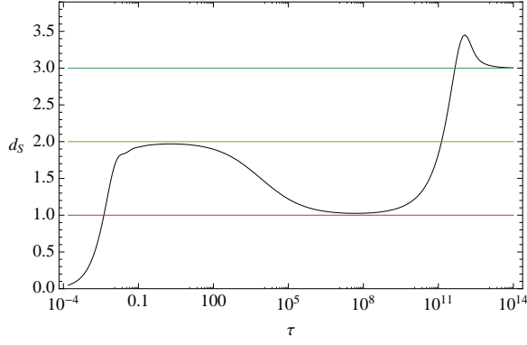
FIG. 5. Spectral dimension of superpositions with coefficients |c_j|^2 = j^{-4} + 200j^{-7} summing from j_{\min} = 1/2 to j_{\max} = 200 for d = 3 and \beta = 3 (to be able to numerically cover enough scales with a feasible number of states in the sum). According to (17), two different UV regimes with dimension d_s \approx 2 and then d_s \approx 1 can be observed.
