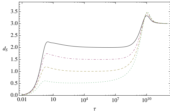
FIG. 2. Spectral dimension of superposition states \alpha = 1/2, 1, 3/2, 2 (dotted, dashed, dot-dashed, solid curve) in d = 3 with cutoff j_{\max} = 10^5 .
