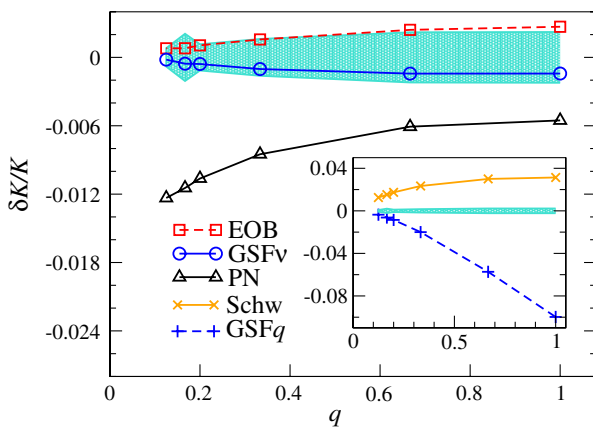
FIG. 3 (color online). The relative difference \delta K/K = (K - K_{\text{NR}})/K_{\text{NR}} as a function of the mass ratio q , for m\Omega_\phi = 0.022 . The PN and EOB results are valid at 3PN order. The shaded area marks the error margin of the NR data. The results are qualitatively identical and quantitatively similar for other values of \Omega_\phi .
