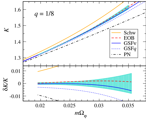
FIG. 2 (color online). The same as in Fig. 1, but for a mass ratio q = 1/8 . Note that for an orbital frequency m\Omega_\phi \sim 0.03 , corresponding to a separation r \sim 10m , the periastron advance reaches half an orbit per radial period.
