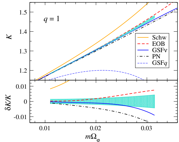
FIG. 1 (color online). The periastron advance K of an equal mass black-hole binary, in the limit of zero eccentricity, as a function of the orbital frequency \Omega_\varphi of the circular motion. The NR results are indicated by the cyan-shaded region. The PN and EOB results are valid at 3PN order. The lower panel shows the relative difference \delta K/K \equiv (K - K_{\text{NR}})/K_{\text{NR}} .
