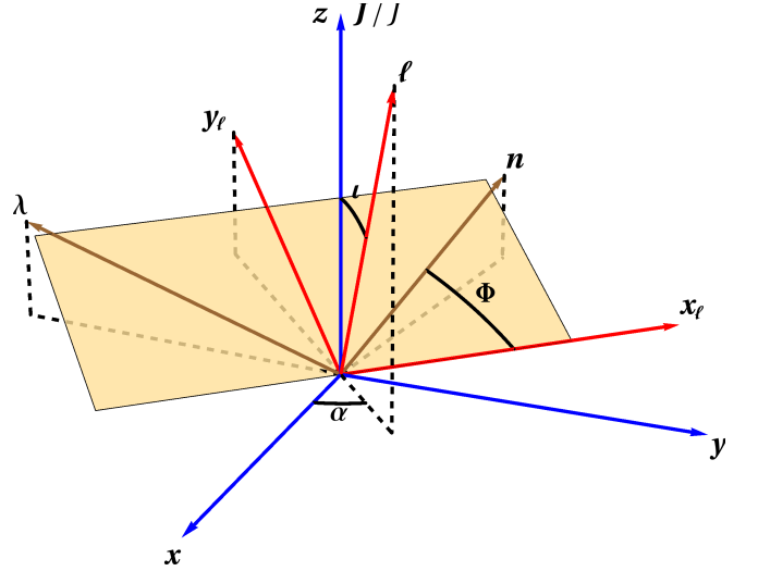
FIG. 1: We show (i) the source frame defined by the orthonormal basis (\mathbf{x}, \mathbf{y}, \mathbf{z}) , (ii) the instantaneous orbital plane which is described by the orthonormal basis (\mathbf{x}_\ell, \mathbf{y}_\ell, \boldsymbol{\ell}) , (iii) the moving triad (\mathbf{n}, \boldsymbol{\lambda}, \boldsymbol{\ell}) , and (iv) the direction of the total angular momentum \mathbf{J} (agreeing by definition with the z -direction). Dashed lines show projections into the x - y plane.
