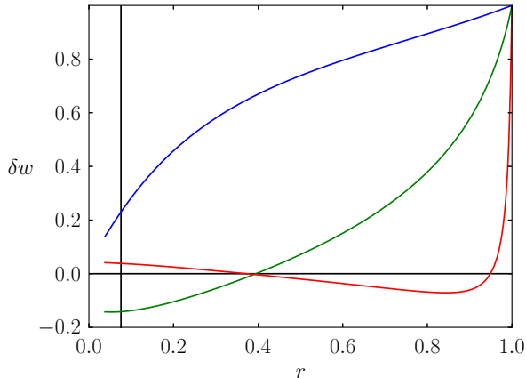
FIG. 1. The first three unstable eigenmodes of the Reissner-Nordström solution as a function of conformal radius r . The horizon radius R_h = 2.57 and slicing constant C_h = -1.84 in (25) have been chosen to agree with the attractor observed in the evolutions of Sec. IV B. The modes have been normalized so that \delta w = 1 at \mathcal{I}^+ . The location of the horizon is indicated by the vertical black line.
