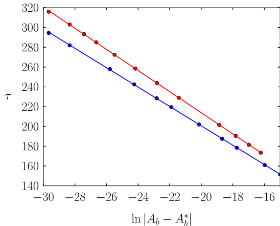
FIG. 9. The time t = \tau when the evolution departs from the critical solution as a function of the logarithm of the parameter distance in A_b -critical searches. The blue line is for r_b = 0.7 , where the critical solution is a colored black hole, whereas the red line is for r_b = 0.6036 \approx r_b^* , where the critical solution is the Reissner-Nordström black hole. The lines are linear fits to the data points.
