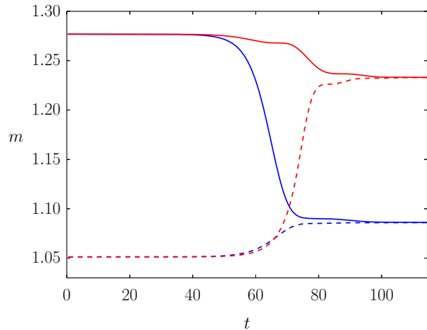
FIG. 3. Bondi mass m_{\mathcal{G}+} (solid lines) and apparent horizon mass m_h = \frac{1}{2}R_h (dashed lines) as functions of time for two perturbed colored black hole evolutions with opposite sign of the perturbation: blue lines correspond to a final vacuum state w = -1 , red lines w = +1 . The initial horizon radius is R_h = 2.11 (chosen to agree with the attractor of the evolution with r_b = 0.7 in Sec. IV B).
