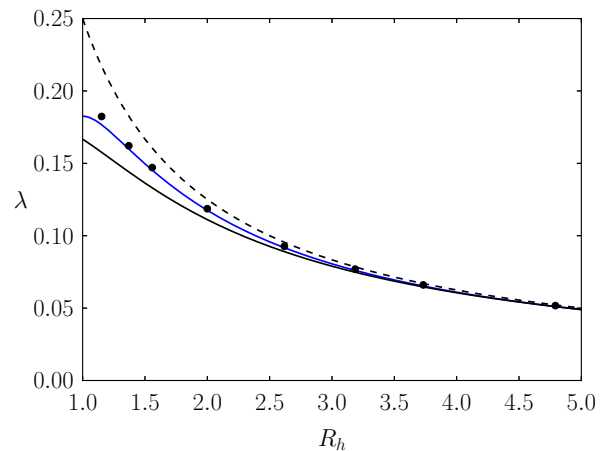
FIG. 2. Top: the first three unstable eigenvalues of the Reissner-Nordström solution as functions of horizon radius R_h . The colors correspond to Fig. 1. Bottom: comparison of the dominant eigenvalue (blue) with Hod's bound [27] in its weak (dashed black) and strong (solid black) form, where for the latter we take \Delta\mathcal{E} to be the entire mass outside the horizon. If instead \Delta\mathcal{E} is taken to be the fraction of this mass that falls into the black hole in a nonlinear evolution, the black points result.
