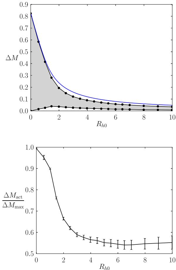
FIG. 4. Masses of colored black holes and their decay products. In the top panel, the blue line shows the total mass of hair \Delta M_{\text{max}} = M - \frac{1}{2}R_{h0} outside the horizon radius R_{h0} of the initial colored black hole. The upper black line represents the quantity M_{f+} - \frac{1}{2}R_{h0} , where M_{f+} is the mass of the final Schwarzschild black hole in a w \rightarrow +1 evolution. The lower line shows the corresponding M_{f-} - \frac{1}{2}R_h for a w \rightarrow -1 evolution. The difference \Delta M_{\text{act}} = M_{f+} - M_{f-} is the actual mass gap, indicated by the shaded region. The ratio of the actual and the maximal mass gap is plotted in the lower panel. The error bars indicate an estimate of the numerical accuracy.
