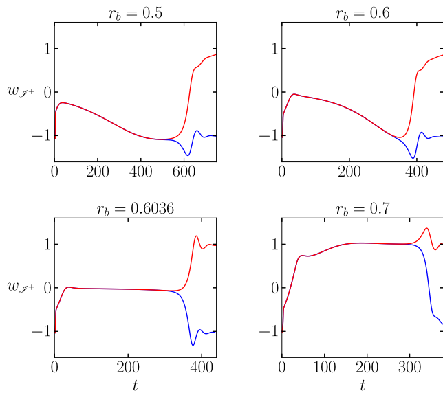
FIG. 7. A_b -near-critical evolutions of w at future null infinity for a few typical values of r_b . The value of A_b for the slightly subcritical (blue) and slightly supercritical (red) evolutions differs by \approx 10^{-14} .
