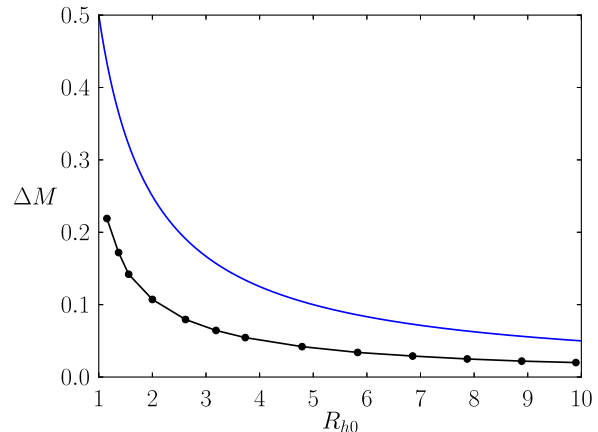
FIG. 5. Masses of Reissner-Nordström black holes and their decay products. The blue line shows the mass of the Yang-Mills field outside the horizon radius R_{h0} of the initial Reissner-Nordström black hole, \Delta M_{\text{max}} = M - \frac{1}{2}R_{h0} . The black line represents the quantity M_f - \frac{1}{2}R_{h0} , where M_f is the mass of the final Schwarzschild black hole.
