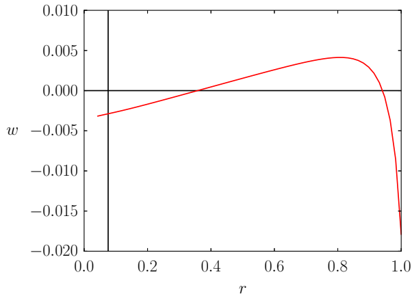
FIG. 12. The Yang-Mills potential w as a function of conformal radius r at time t = 250 for an evolution with r_b = 0.6036 \approx r_b^* . Compare with Figs. 1 and 7.
