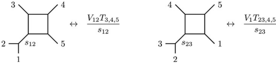
Figure 4 The explicit superspace representation of the five-point box numerators. The form of the numerators depends on the location of leg 1, and the origin of this difference is due to the string one-loop amplitude prescription (18) fixing the position of its first vertex operator V_1 .
