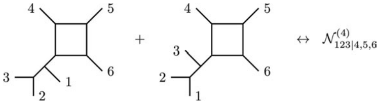
Figure 6 The pure spinor superspace description of two one-mass box graphs in the six-point amplitude is compactly captured by Berends–Giele numerators such as \mathcal{N}_{123|4,5,6}^{(4)} defined in (46). The expansion of the above superspace expression is given in (50).
