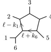
Figure 7 Diagrammatic justification for the shift of loop momentum in \mathcal{N}_{61|2,3,4,5}^{(5)}(\ell + k_6) : The shifted momentum \ell + k_6 occurs in the pentagon edge adjacent to the tree-level subdiagram subtending particles 6 and 1.
