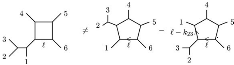
Figure 11 Counterexample for kinematic Jacobi relations at six points in the particular representation of section 4.4.
