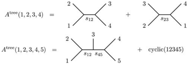
Figure 3 The four- and five-point tree amplitudes represented in terms of cubic graphs.
