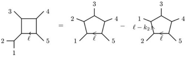
Figure 10 Kinematic Jacobi relations relate pentagon numerators to box numerators.
