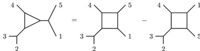
Figure 9 Kinematic Jacobi relations relate box and triangle numerators. Since maximally SYM amplitudes are not expected to contain triangles (nor bubbles and tadpoles), the left-hand side must vanish.
