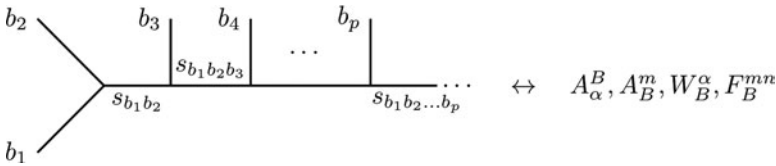
Figure 1 The correspondence of cubic graphs and the BRST blocks with multiparticle label B = b_1 b_2 \dots b_p . For the unintegrated vertex V_B = \lambda^\alpha A_\alpha^B , this mapping implies that the BRST variation of cubic graph numerators cancels propagators and allows the construction of BRST invariant tree-level amplitudes.
