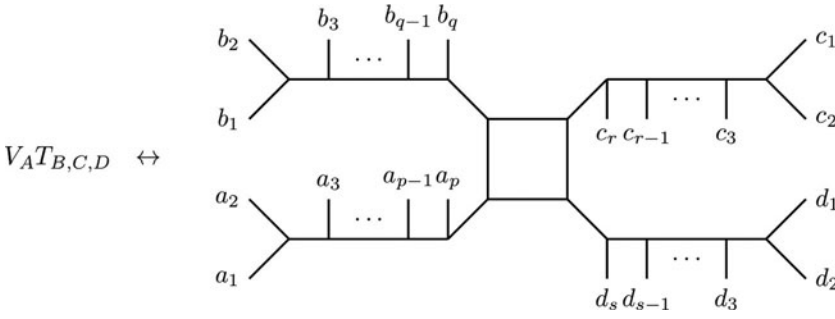
Figure 5 On-shell diagrams represented by V_A T_{B,C,D} connect four off-shell subdiagrams. Propagators such as s_{a_i a_j} and s_{a_i a_j a_k} are suppressed on the left-hand side.
