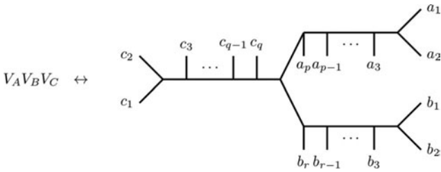
Figure 2 On-shell diagrams represented by V_A V_B V_C connect three off-shell subdiagrams. Propagators such as s_{a_1 a_2} and s_{a_1 a_2 a_3} are suppressed on the left-hand side.
