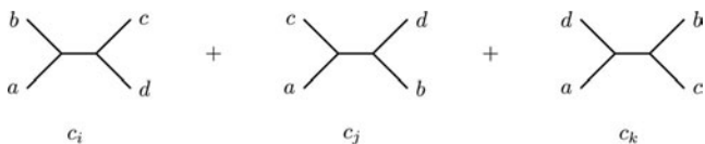
Figure 8 The vanishing of the color factors associated to the above triplet of cubic graphs, c_i + c_j + c_k = 0 is a consequence of the Jacobi identity. In the above diagrams, the legs a, b, c and d may represent arbitrary subdiagrams. The BCJ duality states that their corresponding kinematic numerators N_i can be chosen such that N_i + N_j + N_k = 0 .
