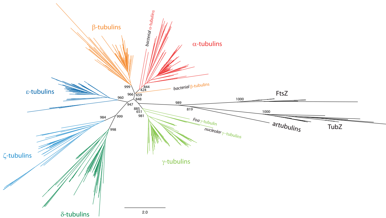
Fig. 1. —Phylogenetic tree of the tubulin protein family. Unrooted ML topology generated under the WAG + \Gamma model in FastTree showing branch lengths for 75 \alpha -, 69 \beta -, 84 \gamma -, 50 \delta -, 45 \epsilon -, 32 \zeta -tubulins, 2 bacterial tubulins, 1 “artubulin,” 11 bacterial FtsZ, and 8 bacterial TubZ proteins. CD-Hit (70% identity) was used to obtain a representative data set for subfamily classification and visualization. Support for the major branchings indicating the grouping of the tubulins and FtsZ family members into different subtypes is given as likelihood bootstraps (FastTree). The scale bar corresponds to estimated amino acid substitutions per site.
