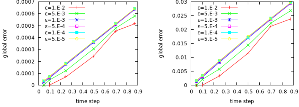
FIGURE 6. First nonlinear case, Algorithm 4.1 with the particles mean period: the global Euclidean error at time 3.5 for an initial particle on (left) and off (right) the slow manifold
