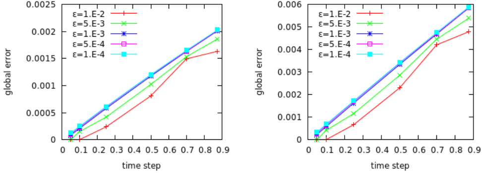
FIGURE 7. Vlasov-Poisson case, Algorithm 4.1 with the particles mean period: the global Euclidean error at time 3.5 for an initial particle on (left) and off (right) the slow manifold
