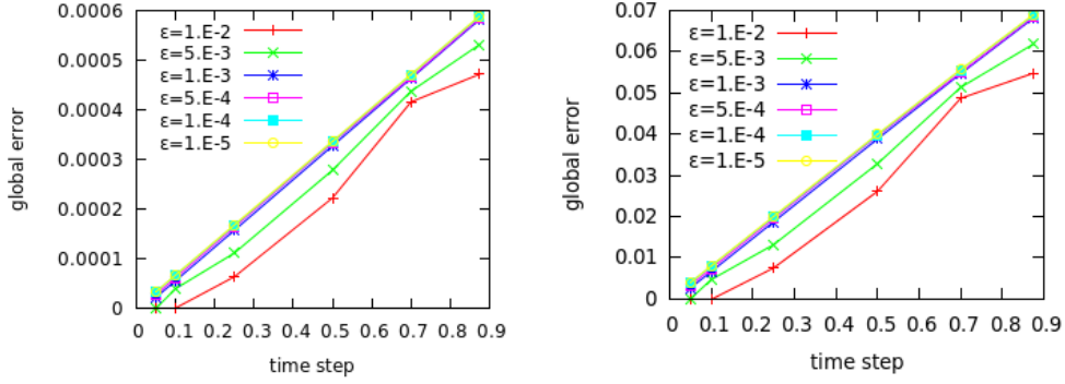
FIGURE 3. First nonlinear case: the global Euclidean error at time 3.5 for an initial particle on (left) and off (right) the slow manifold
