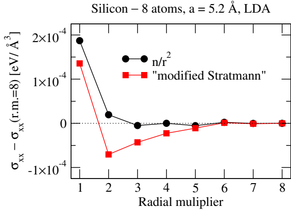
Figure 9: Change of the analytical stress for increasing integration grid densities relative to the densest used grid. The behavior for two different integration partition functions is shown, see text. Increasing the radial multiplier increases the number of spherical integration shells around every atom, and therefore, leading to a denser integration grid. For more details about the used integration grid see Appendix D.1. The calculations were performed for a diamond unit cell of silicon (8 atoms) with the LDA functional at a lattice parameter of 5.2 Å.
