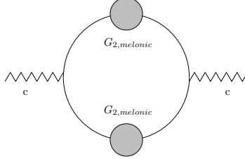
Figure 14: A melonic two point insertion
