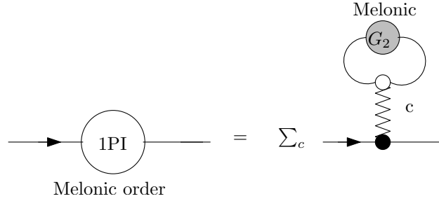
Figure 12: 1PI melonic two point function
