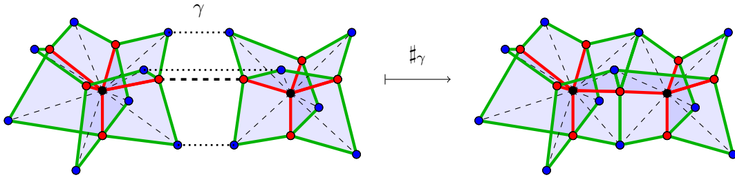
Figure 2: The bonding \sharp_\gamma of two atoms along an identification of patches \gamma .
