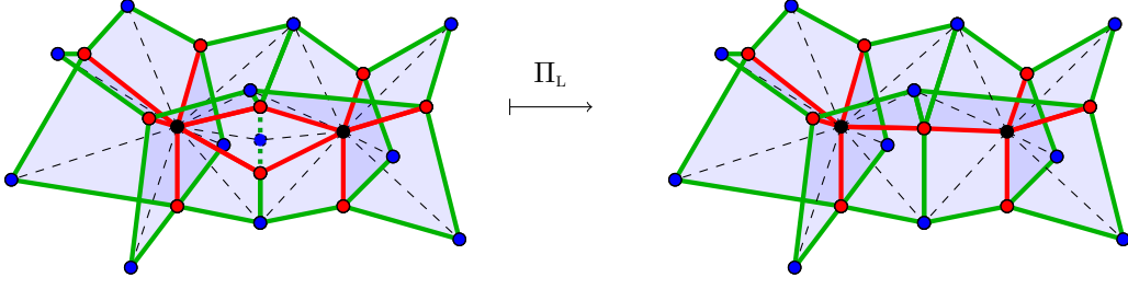
Figure 4: Contraction move with respect to a vertex \hat{v} incident to two virtual edges in a molecule.
