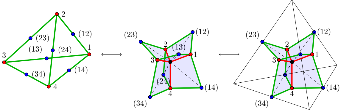
Figure 1: A bisected k -regular graph, its corresponding spin foam atom, and a k -dimensional extension which, in this example, is the dual of the tetrahedron.
