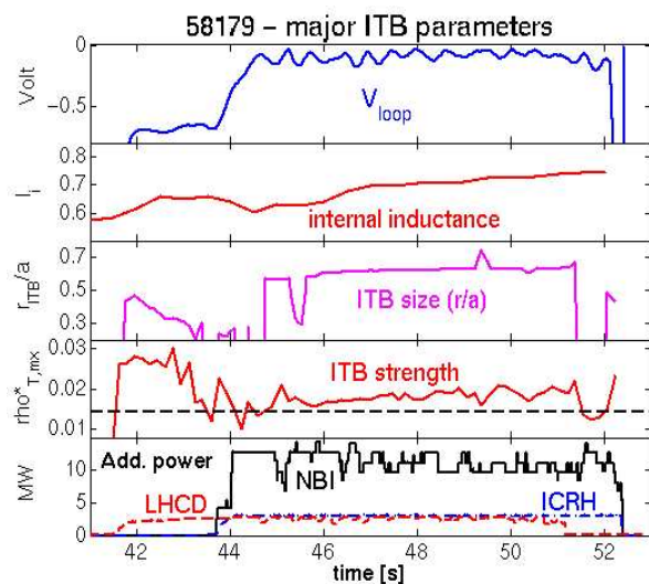
Fig. 1. Long lasting ITB: time evolution of the main quantities. For this particular pulse E_{inj}=150 MJ
