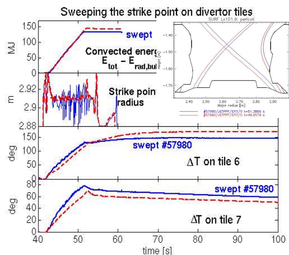
Fig. 4. Comparison of the divertor tiles behaviour w/w.o. the strike point sweeping. In the insert: the divertor legs with the two extreme positions of the separatrix during the sweeping
