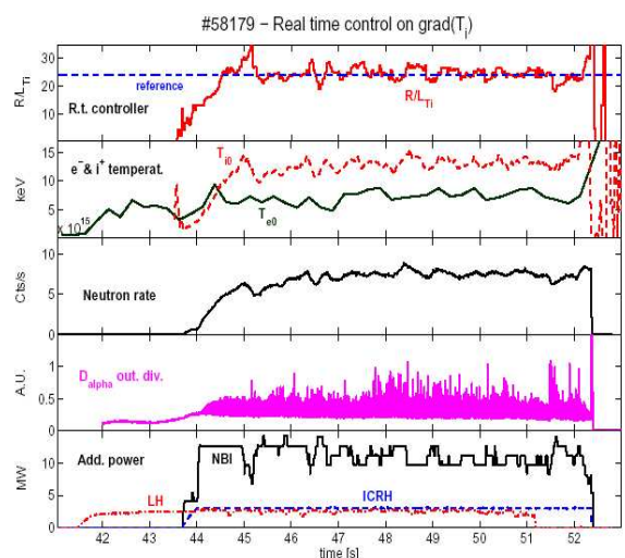
Fig. 2. Time evolution of the main quantities during a real time controlled, long lasting ITB
