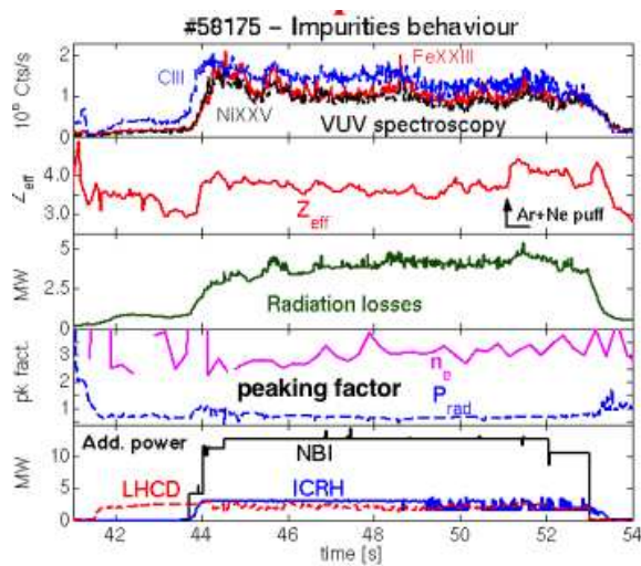
Fig. 3. Time behaviour of the most relevant plasma parameters referring to impurities
