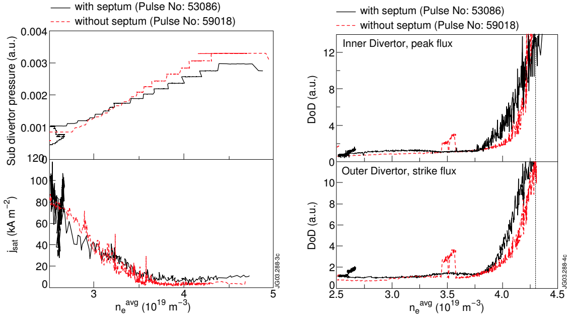
Figure 2: Left: comparison of sub-divertor pressure and ion saturation current at inner strike zone, with and without septum, main chamber fuelling; Right: comparison of DoD with and without septum, main chamber fuelling.
