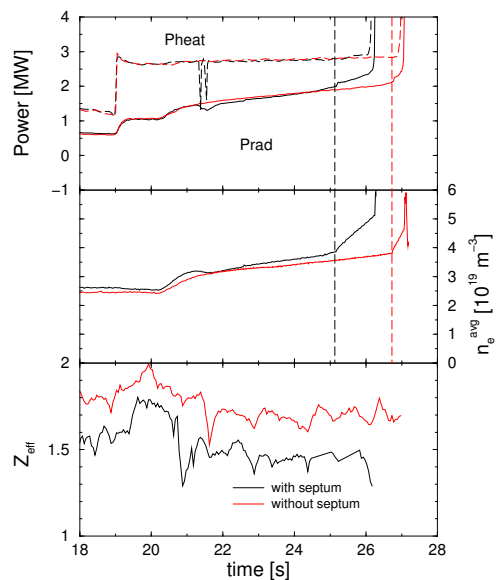
Figure 1: Comparison of L-mode density limit discharges (53080 w septum, 58718 wo septum) 1.7MA/2.4T, P_{NBI} = 2MW
