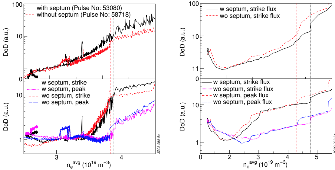
Figure 3: Left: DoD for inner divertor with septum (53080) and outer without septum (58718); Right: Simulation of detachment (DoD) in density limit discharges with EDGE2D/NIMBUS; X-point MARFE onset is indicated by the dashed line.
