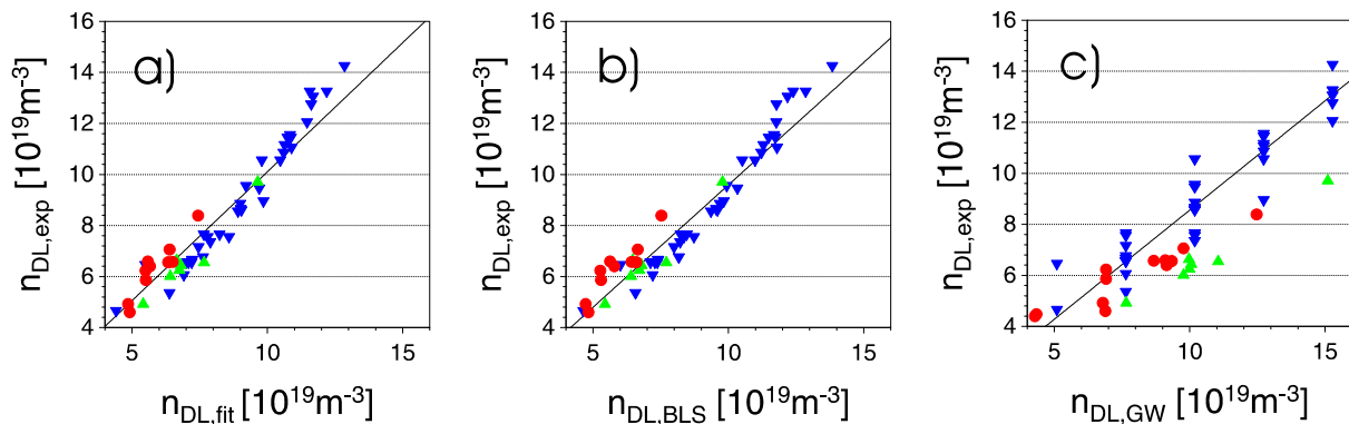
FIG. 3. Experimental density limit n_{DL,exp} (Lidar) versus n_{DL,fit} (a), n_{DL,BLS} (b) and Greenwald density n_{DL,GW} (c). Experimental data are from JET Mark-I and Mark-II (upward triangles), the gas box divertor configuration (bullets) and from the ASDEX Upgrade Divertor II configuration (downward triangles). Within the database the variations of P_h , B_t and q_{95} cover the ranges 3.5–19.5 MW, 1.0–3.5 T and 2.5–11.5, respectively.
