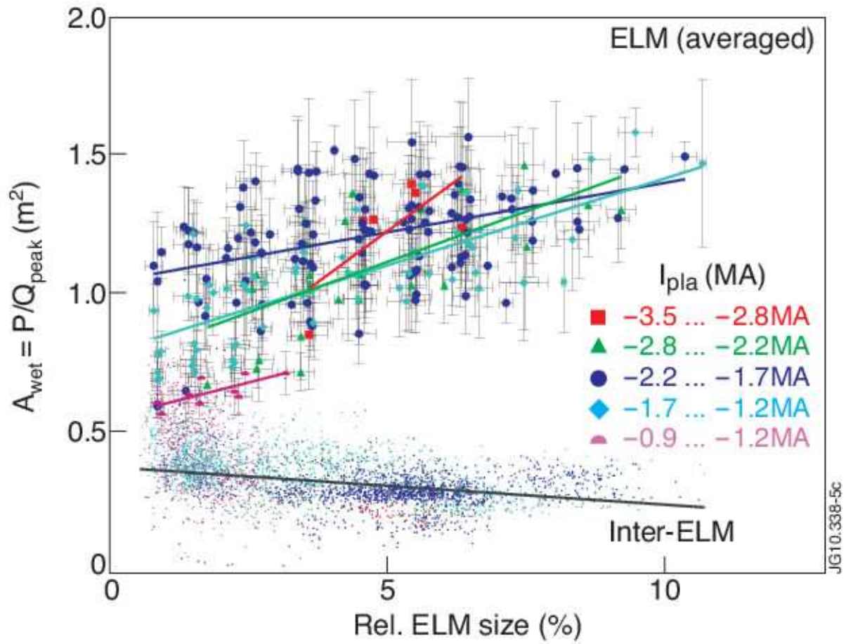
FIG 4: Database of wetted area versus the ELM size normalized to W_{\text{MHD}} . Different colours indicate plasma current intervals (negative plasma currents I_p correspond to the regular magnetic configuration in JET) and solid lines denote linear fits to the wetted area in the respective interval.
