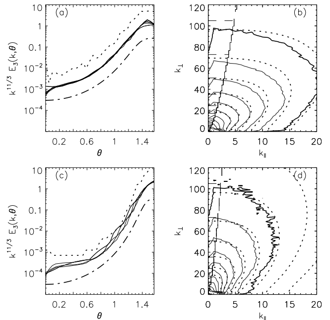
FIG. 5: Anisotropy in ideal runs; (a-b) B_0 = 5 (c-d) B_0 = 10 . (a)-(c): k_d^{11/3} (dotted), k^{11/3} E_3(k, \theta) (solid) (a) for 6 \leq k \leq 12 and (b) for 5 \leq k \leq 8 , Eq.(7) (dashed-dotted) with m = 5/3 , and (a) \varepsilon = 0.158 (c) \varepsilon = 0.158/2 . (b)-(d): energy contour levels of E_3(k_{\parallel}, k_{\perp}) : simulation data (solid); Eq. 2 (dashed line, the oblique line tracing the boundary \chi = 1 with k_0 = 5 , B_0 = 5 (b) and B_0 = 10 (d)); Eqs. 3,7 with \beta = 3 , \varepsilon = 0.158 (b) and \varepsilon = 0.158/2 (dotted)
