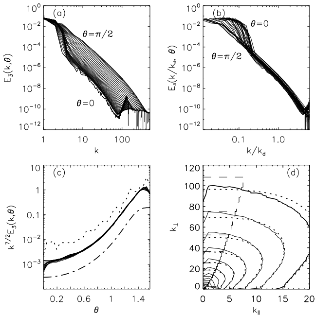
FIG. 3: Details of spectral properties: (a) E_3(k, \theta) for \theta ranging from 0 to \pi/2 , (b) E_3(k/k_d, \theta) (c) k_d^{7/2} (dotted), k^{7/2} E_3(k, \theta) for 8 \leq k \leq 20 (solid), Eq.(7) with m = 3/2 (dotted-dashed) (d) energy contour levels of E_3(k_{\parallel}, k_{\perp}) : simulation data (solid); Eq. 2 (dashed line, the oblique line tracing the boundary \chi=1 with k_0 = 5 , B_0 = 5 ); Eqs. 3,7 with \beta = 3 , \varepsilon = 0.158 (dotted)
