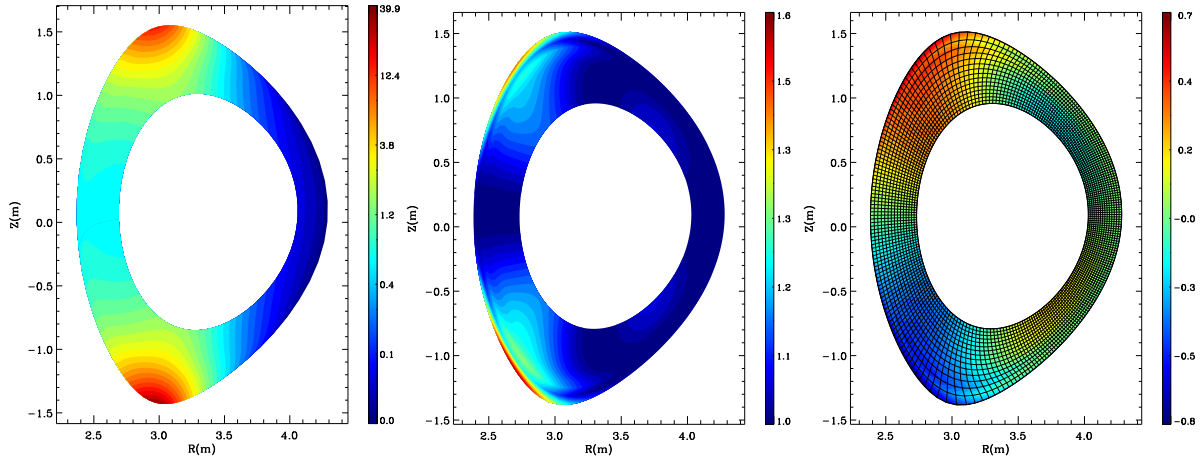
Figure 1: Conformal ratio for an ASDEX Upgrade based equilibrium computed with the HELENA MHD solver. The radial domain shown is 0.65 < \rho_{\text{tor}} < 0.96 in units of normalised toroidal magnetic flux for (left) Hamada coordinates and (center) conformal coordinates. (right) conformal grid and associated shear deformation d .
