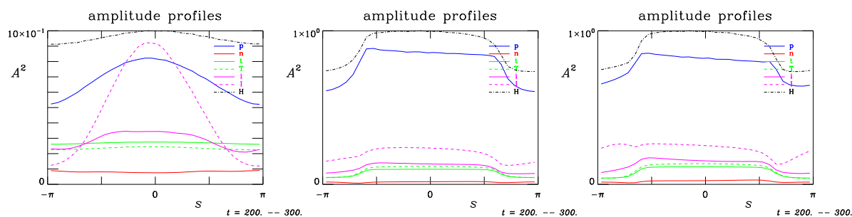
Figure 2: Squared amplitude envelope of the (blue) electrostatic potential, (red) electron density, (green) electron temperature, (magenta) ion temperature and (black) nonadiabatic density fluctuations along the parallel coordinate.
