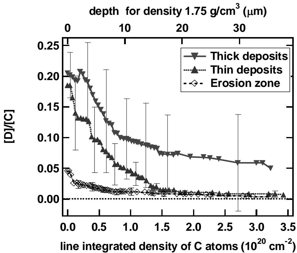
Figure 6: Average [D]/[C] ratio deduced from NRA measurements vs. line integrated density of C atoms (bottom axis) and depth (assuming a carbon density of 1.75 \text{ g/cm}^3 , top axis) for Thick deposits, Thin deposits and Erosion zones. Vertical bars show the dispersion from sample to sample. The surface roughness is \sim 5 \mu\text{m} .
