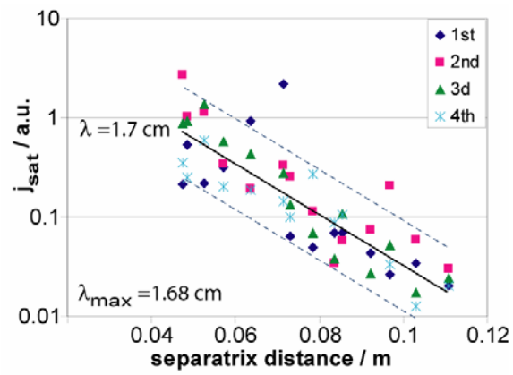
Fig. 4 E-folding lengths for the first 4 filaments in an ELM as measured with the reciprocating probe.
