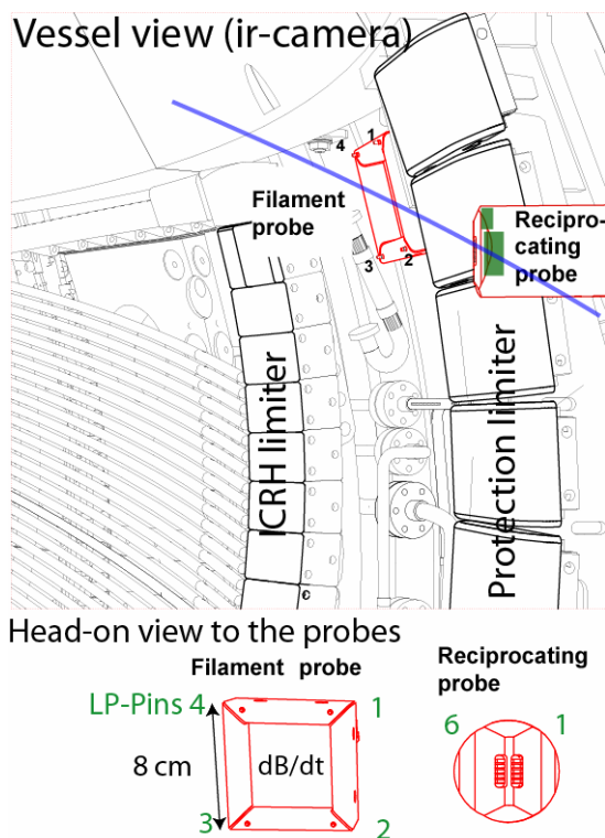
Fig. 1 Langmuir and magnetic pick-up probes in the field of view of the ir-camera located above the outer mid-plane of ASDEX Upgrade. The regions which were used for the heat flux plots and the names of the probes are marked. The line indicates a magnetic field line. The toroidal separation of the probes is about 0.6 m.
