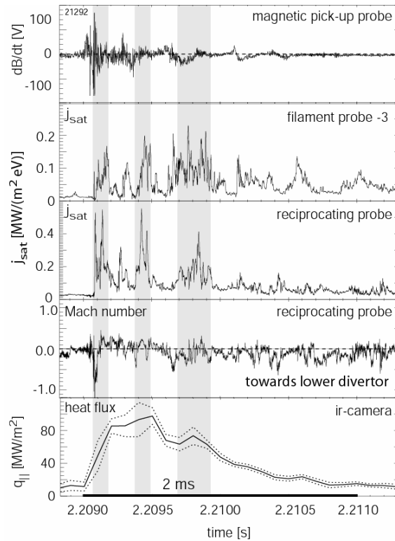
Fig. 2 Time slices of measurements during a single ELM with the probes from Fig. 1. The Mach number was calculated from pin 1 and 6 of the reciprocating probe. The heat flux is the mean value of the center region at the probe head with the dashed lines showing the standard deviation. The grey bars mark single filaments for better comparison.
