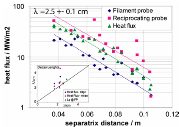
Fig. 3 Heat flux decay lengths as measured by Langmuir probes at two different toroidal positions and by thermography. A factor of \gamma T_e = 100 eV is assumed to derive the heat flux from the ion saturation current. The inset shows all e-folding lengths measured by the filament probe and by thermography vs. the reciprocating probe results.
