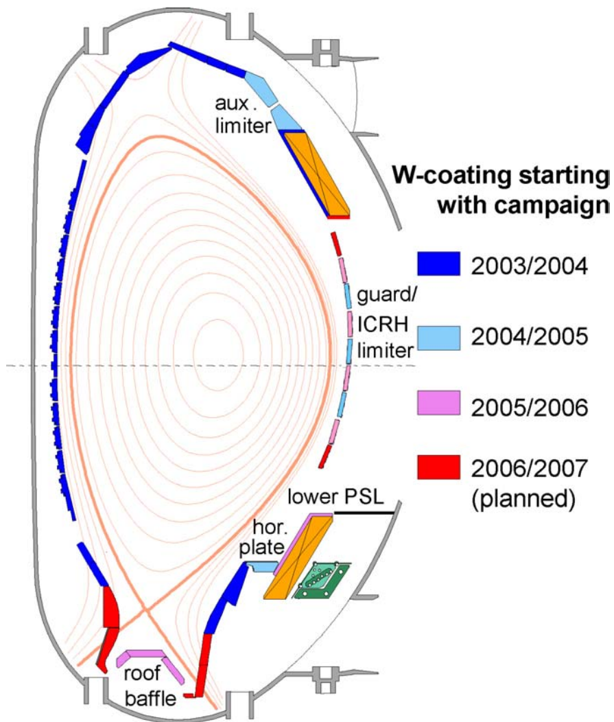
Figure 1: Poloidal cross section of ASDEX Upgrade with colour coded PFCs representing the time of implementation of W coated tiles.
