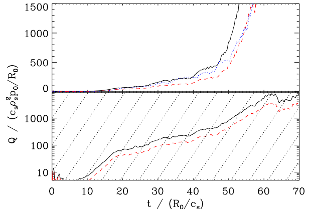
FIG. 1. (Color online) Transport levels Q for \beta = 0.9\% : the black solid, red dashed, and blue dotted lines correspond to the ion and electron electrostatic fluxes, and the electron electromagnetic flux, respectively. Both plots show the same data, the lower on a logarithmic axis, with black dotted lines of a slope twice the maximum linear growth rate, which is not exceeded by the Q s.
