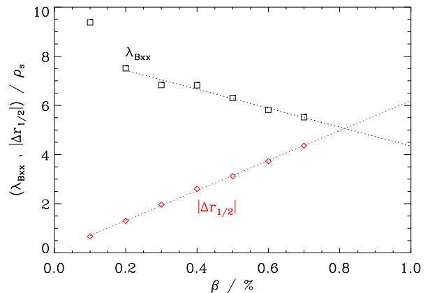
FIG. 3. (Color online) Half-turn radial field line displacement \Delta r_{1/2} and B_x correlation length \lambda_{Bxx} as a function of \beta ; linear fits indicate an intersection just above \beta = 0.8\% .
