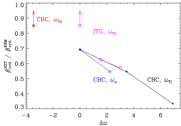
FIG. 2. (Color online) Impact of gradient variations \Delta\omega on \beta_{\text{crit}}^{\text{NZT}} (normalized to \beta_{\text{crit}}^{\text{KBM}} ) for CBC and ITG case parameters. Different symbols/colors indicate different gradients. Vertical arrows signify that for a particular \Delta\omega , the NZT threshold lies above the ballooning threshold.
