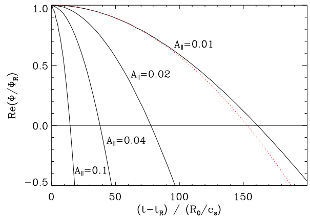
FIG. 4. (Color online) Zonal flow decay in the presence of various values of a resonant and time-independent A_{\parallel} \propto B_x . Shown is the real part of the electrostatic potential \Phi relative to the residual \Phi_R (with \text{Im}(\Phi) \ll \text{Re}(\Phi) ); time is measured relative to t_R where the residual had been reached ( B_x is turned on t = t_R ). The dotted red line shows an exemplary quadratic fit to the data, consistent with analytical theory.
