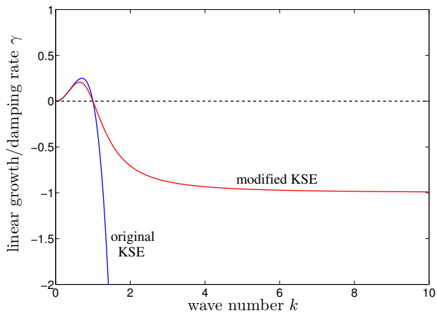
FIG. 1: Linear growth/damping rate \gamma as a function of wave number k for the original and modified Kuramoto-Sivashinski equation. (color online)
