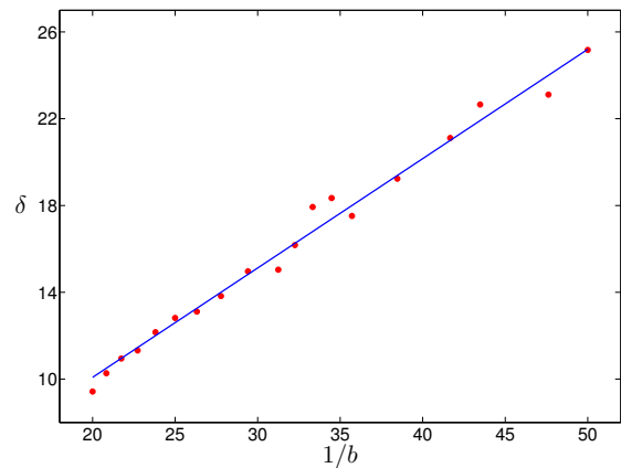
FIG. 5: The exponent \delta = 2\lambda\nu/b in the power law E(k) \propto k^{-\delta} as a function of the damping rate 1/b for \nu = 1 . (color online)
