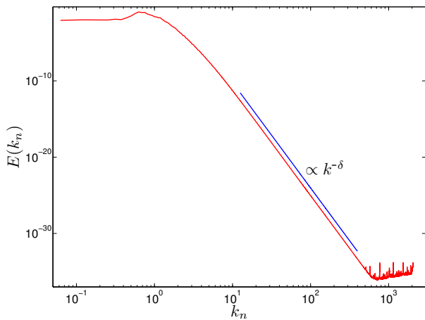
FIG. 4: Fit of a power law (blue line) to the high- k end of the energy spectrum (red line) for b = 0.036 . (color online)
