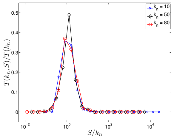
FIG. 2: Net energy transfer into mode k_n via triads with the scale disparity parameter S as a function of S normalized to k_n . (color online)
