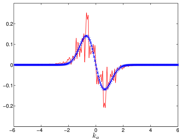
FIG. 3: Triple correlation normalized to E(k_n + k_q^{min}) (red line) as a function of k_q for k_n = 50 and b = 0.036 compared to the model f_P(k_q)/E(k_n + k_q^{min}) denoted by blue crosses. (color online)
