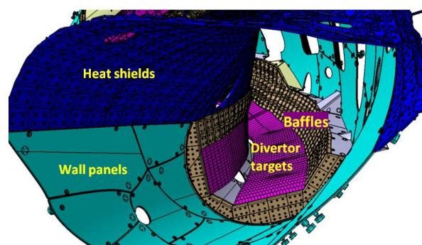
Fig. 1. PFCs, toroidal view at triangle cross-section
