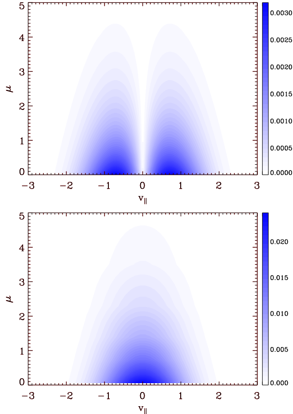
FIG. 5. (Color online) Ion distribution function |f| in velocity space for the standard initial condition IC1 (top) and the alternate version IC2 (bottom) designed to obtain cleaner results with less computational effort. Both plots represent snapshots after the respective oscillating phase has died down, at the moment when B_x is turned on. The difference does not influence zonal flow decay due to B_x , however: the specific shape of the ion distribution does not enter into the analytical calculation. The corresponding electron distributions are almost identical qualitatively for both initial conditions.
