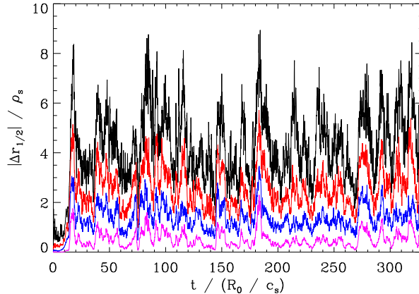
FIG. 9. (Color online) Radial displacement \Delta r_{1/2} of field lines as a function of time, at the outboard midplane for CBC parameters at \beta = 0.7\% . From top to bottom, the curves correspond to the displacement exceeded by the most-displaced field line (black), the 10% most-displaced field lines (red), the e-fold fraction (blue), and the average displacement of all lines (pink). For these curves, 1000 lines were traced.
