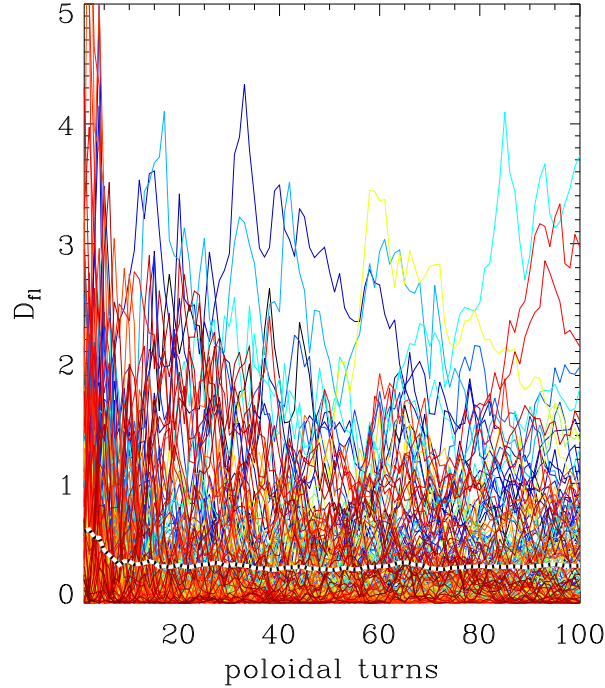
FIG. 8. (Color online) Field line diffusivity as a function of the poloidal turn number; different colors correspond to different field lines. The black-and-white dotted line marks the average over field lines: after an initial phase where lines move ballistically, the stochastic (diffusive) regime is reached, and D_{fl} saturates. See the caption of Fig. 7 for more details.
