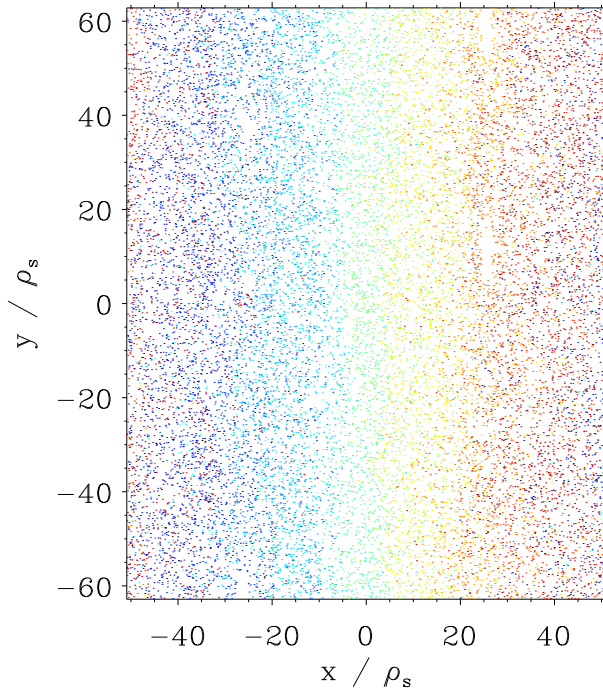
FIG. 7. (Color online) Poincaré section (inboard midplane) for the same simulation data as in Fig. 9 at t = 328.8 . Different colors correspond to different seed positions of the field lines (all seeded at y = 0 ), out of a total of 200 lines traced for 100 poloidal turns. The mixing of colors indicates a strongly stochastic field.
