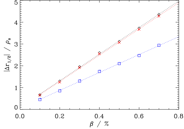
FIG. 12. (Color online) Half-turn field line displacements \Delta r_{1/2} of the most-displaced lines as functions of \beta for the unmodified simulation data (black diamonds); with even-parity A_{\parallel} filtered out for k_x = 0 and connected k_x (red crosses); and with even-parity A_{\parallel} filtered out for all k_x (blue squares). The reduction (but not elimination) of the displacement in the two latter cases (especially the last one) supports the concept of SMT catalyzation (see the text).
