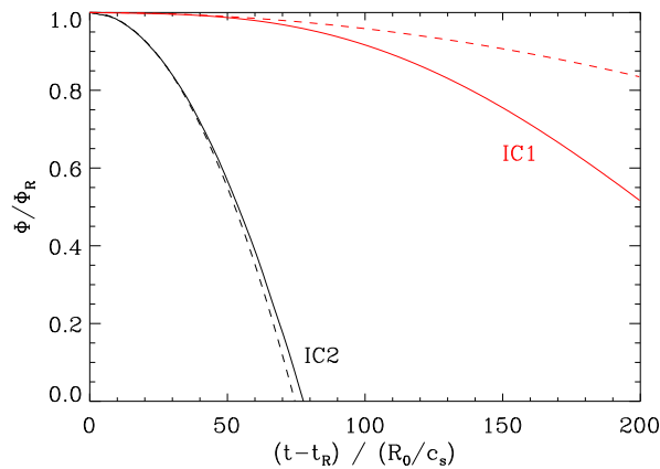
FIG. 4. Decay of the zonal flow residual due to resonant magnetic fluctuations, for two different initial conditions labeled IC1 (red) and IC2 (black), see the text. Here, the initial oscillatory phases were computed without B_x , and moderate collisionality and/or v_{\parallel} hyperdiffusion were used during t < t_R to reduce the velocity space fine structure more quickly. A quadratic fit (dashed curves) was obtained for IC2 which also applies to IC1 when rescaled appropriately, see the text. Both curves start to deviate from the quadratic fit curves near t - t_R \approx 70R_0/c_s .
