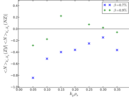
FIG. 13. (Color online) Free energy transfer due to zonal flow coupling \sum_{kx'} \mathcal{N}_{(kx, ky), (kx', ky'=ky, 0)} (normalized to the total non-zonal energy transfer) for \beta < \beta_{\text{crit}}^{\text{NZT}} (blue crosses) and \beta > \beta_{\text{crit}}^{\text{NZT}} during the runaway phase (green pluses). The negative values for the former case indicate energy transfer via the zonal flows to higher k_x , consistent with the zonal flow shearing paradigm. In the latter case, the zonal coupling is much weaker or even positive, illustrating that the zonal flow dynamics are fundamentally altered and now contribute to the growth at some k_y .
