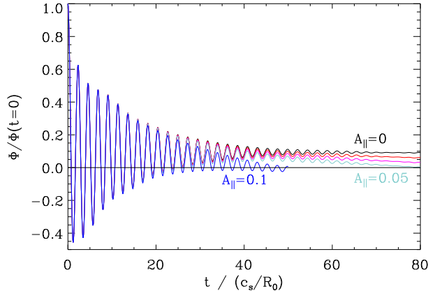
FIG. 2. (Color online) GAM oscillations and zonal flow damping for various, increasing values of the resonant, artificially imposed A_{\parallel} . Shown is the electrostatic potential as a function of time, normalized (separately for each curve) to its value at t = 0 . Stronger magnetic fluctuations result in faster decay of the residual, with the linear dependence predicted by Eq. (1) visible in the simulation data. For A_{\parallel} = 0 , the usual residual \Phi_R is retained.
