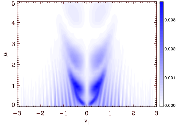
FIG. 3. (Color online) Ion distribution function |f| in velocity space (not the entire \mu domain is shown here), at the outboard midplane. The fine structure dominating the plot is a result of the GAM oscillations (see also Ref. [25]), and the need to resolve it can make simulations rather expensive. This snapshot was taken from the simulation labeled A_{\parallel} = 0 in Fig. 2 at t = 37.4R_0/c_s ; for the curve with the smallest finite A_{\parallel} , the plot for |f| is visually indistinguishable from the one shown here.
