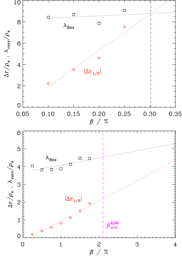
FIG. 11. (Color online) Field line half-turn displacement and radial correlation length of B_x (same nomenclature as in Fig. 10) for GA-standard (upper plot) and TEM case parameters (lower plot). In the first case, the intersection occurs at the NZT threshold (blue dashed line) as expected; whereas in the second it has moved well beyond the KBM threshold (pink dash-dotted line), and no NZT is detected. Both plots use the same definition for \Delta r_{1/2} as in Fig. 10.
