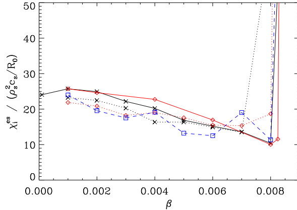
FIG. 1. (Color online) Results from gyrokinetic codes GENE (black crosses), GYRO (red diamonds), and GKW (blue squares) for \beta \leq \beta_{\text{crit}}^{\text{NZT}} : plotted is the ion electrostatic heat diffusivity. The near-vertical lines at the threshold illustrate a transition to very large transport values; for all \beta scans shown, this occurs above \beta = 0.8\% but below \beta = 0.85\% . Good quantitative agreement is found both for the pre-NZT transport and the NZT threshold. Dotted lines (GENE and GYRO) indicate sensitivity tests with slightly different numerical settings.
