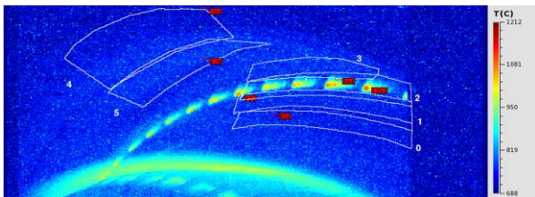
FIG. 1. Image of the divertor view (tangential) taken with the KL11-PIDA camera (JPN82630, frame 1265). The top and bottom of the image show the outer, inner divertor respectively (the view is rotated 90 degrees counter-clockwise). At the centre, the hottest areas correspond to the outer strike point. The white areas superimposed correspond to the ROIs (labeled from 0 to 5) used by the RTPU and the red markers indicate the location and temperature of the validated hot spot.
