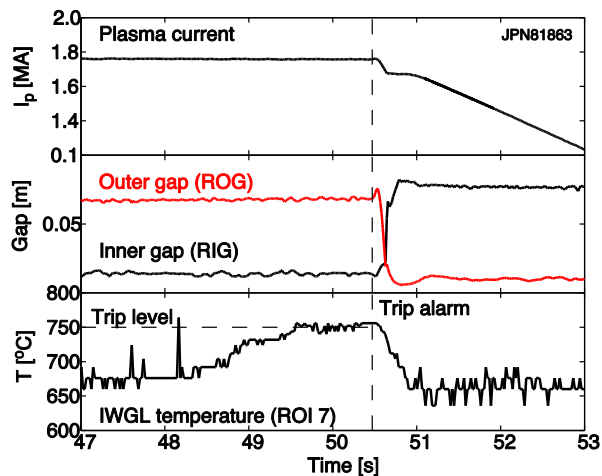
FIG. 2. Evolution of the plasma current, radial outer and inner gaps and temperature output of the RTPU for an ROI monitoring an inner wall guard limiter (IWGL) in a pulse where the trip level is reached and the plasma safely landed.
