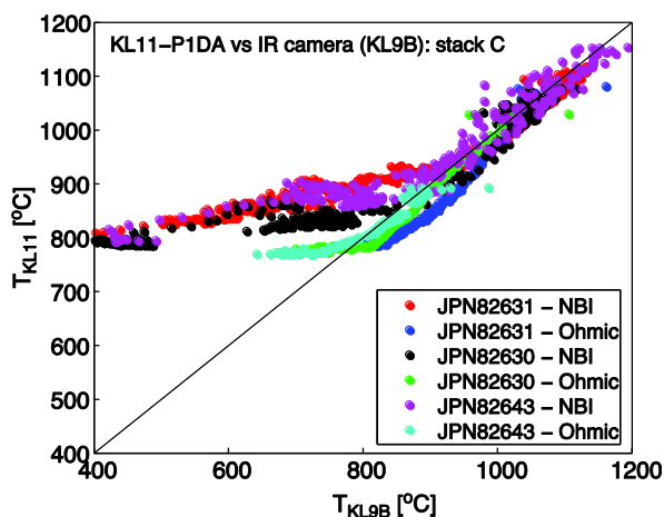
FIG. 3. Real time temperature outputs (ROI 2 of the KL11-P1DA camera) as a function of the temperature measured on a comparable area (stack C of the divertor outer target) by the thermal IR camera (KL9B). Three different plasma pulses, with different fuelling rate are compared. The NBI heating phase is distinguished from the cooling down, ohmic, phase.
