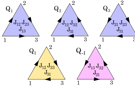
Fig. 2. The triangles indicate the complex structures, whose associated holomorphic curves are solutions of the \sigma -model. The three top triangles correspond to integrable complex structures, whereas the two lower ones correspond to the non-integrable ones. (For interpretation of the references to color in this figure, the reader is referred to the web version of this article.)
