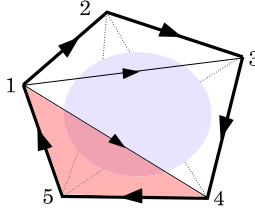
Fig. 1. The procedure showing that a cycle (1, 2, 3, 4, 5) in a graph leads to the violation of condition (10). Using (10), we replace the pair of segments (1, 2), (2, 3) by (1, 3), i.e. cut a corner. Then we replace (1, 3), (3, 4) by (1, 4), arriving at the cyclic lower triangle, which violates (10).
