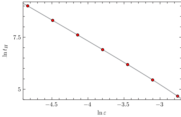
FIG. 1 (color online). Time of horizon formation vs amplitude in the evolution of initial data (14). The solid line depicts the fit of the function -2 \ln \varepsilon + a + b \varepsilon^2 to the numerical data \ln t_H(\varepsilon) . From this fit we obtain \tau_H := \lim_{\varepsilon \rightarrow 0} \varepsilon^{-2} t_H(\varepsilon) = e^a \approx 0.514 .
