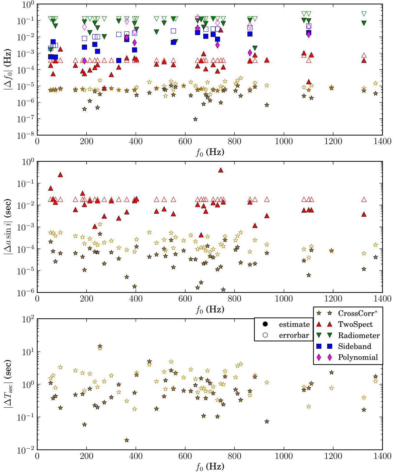
FIG. 5: Comparisons of parameter estimation for detected signal from each pipeline as a function of intrinsic signal frequency.
