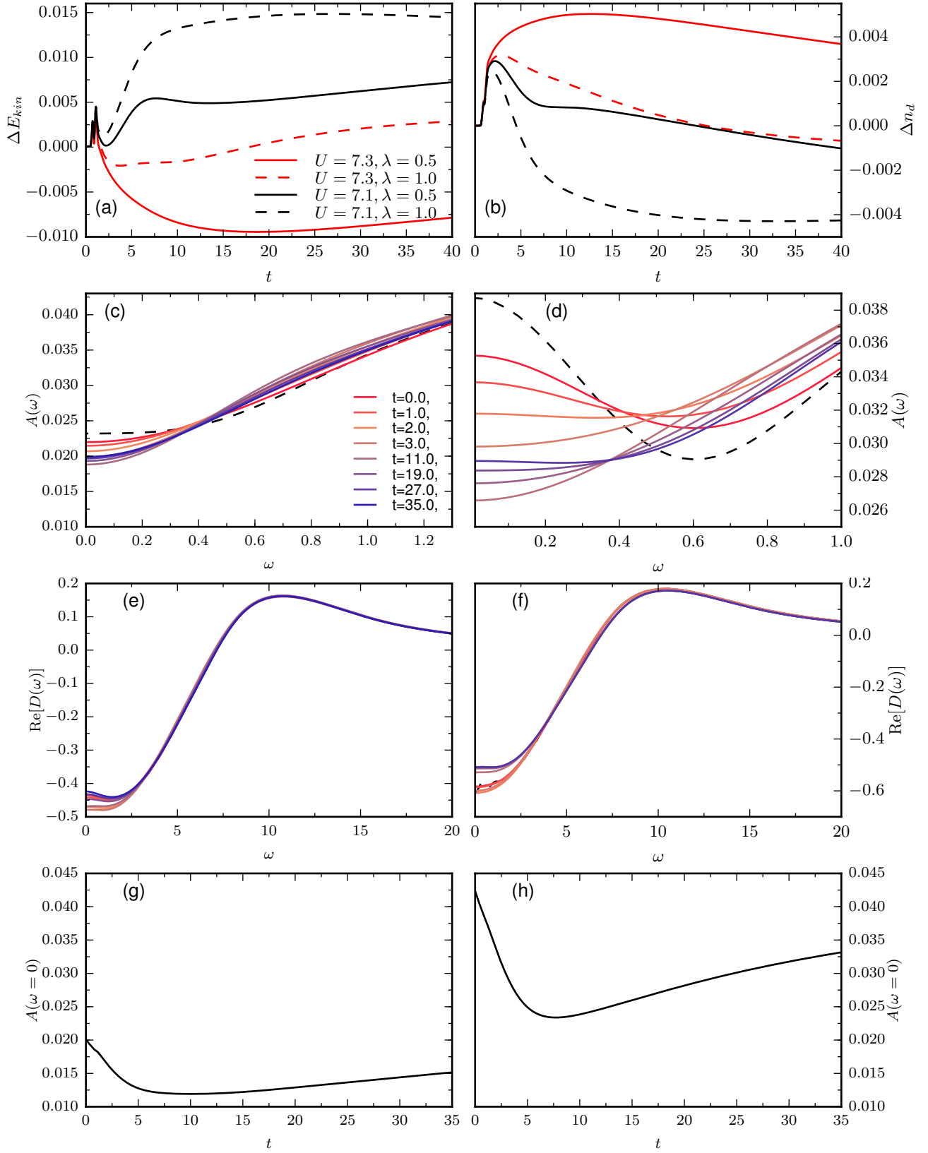
Figure 10. Relaxation dynamics of the kinetic energy E_{\text{kin}} (a) and the double occupancy n_d (b) for U = 7.3 and U = 7.1 at V = 2.0 for different values of the coupling with the bath \lambda = 0.5, 1.0 during and after a pulse with \omega = 8 and E_0 = 1.0 . The partial Fourier transform of the spectral function A(\omega, t) for U = 7.3 and U = 7.1 is shown in panels (c) and (d). The dashed lines corresponds to the equilibrium spectral function. Panels (e,f) plot the real part of the partial Fourier transform of the regular part of the partially screened on-site interaction \text{Re}[D(t, \omega)] = \text{Re}[\mathcal{U}(t, \omega)] - U for U = 7.3 (e) and U = 7.1 (f). The time evolution of the spectral weight A(\omega = 0, t) for U = 7.3 (g) and U = 7.1 (h) for \lambda = 1 .
