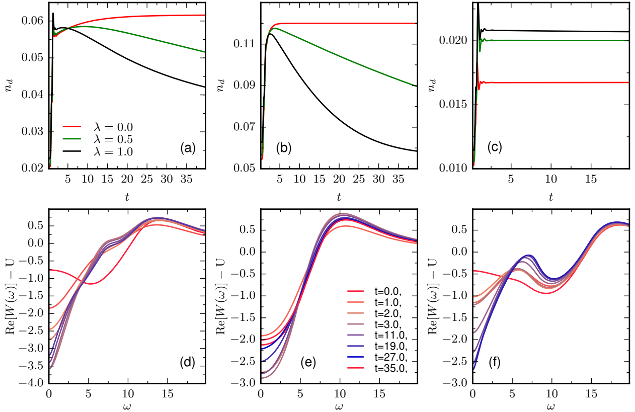
Figure 9. Relaxation dynamics of the double occupancy n_d for U = 7 (a), U = 10 (b), and U = 14 (c) with different values of the coupling to the bath \lambda during and after the pulse with frequency \omega = 8 and pulse amplitude E_0 = 5 . The real part of the partial Fourier transform of the screened interaction \text{Re}[W^{\text{reg}}(t, \omega)] = \text{Re}[W(t, \omega)] - U for U = 7 (d), U = 10 (e) and U = 14 (f) at fixed V = 2.0 , \lambda = 1.0 , E_0 = 5 .
