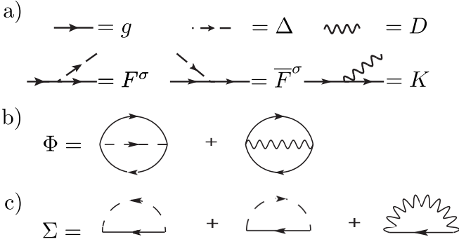
Figure 1. (a) Vertices representing the coupling between pseudo-particle propagators (solid lines) and hybridization functions (dashed lines), or between pseudo-particle propagators and retarded interactions (wavy lines). (b) The lowest order diagrams (in \Delta and \mathcal{D} ) contributing to the Luttinger-Ward functional. (c) The pseudo-particle self-energy diagrams corresponding to the approximation (b) for the Luttinger-Ward functional.
