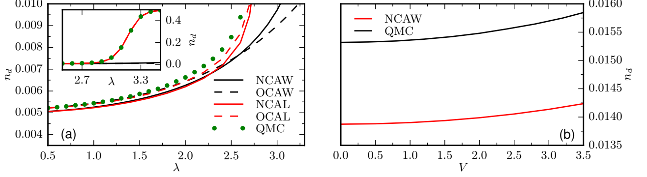
Figure 2. (a) Comparison of the double occupancy in the Holstein-Hubbard model on the Bethe lattice for \beta = 5 , U = 10 , and \omega_0 = 2 obtained from the NCA and OCA approximation in combination with the weak-coupling expansion (W) and Lang-Firsov (L) transformation, and the numerically exact QMC results. (b) Comparison of the double occupancy for the extended Hubbard model for \beta = 5 , U = 12 obtained from the NCA approximation and the numerically exact QMC solver on the square lattice.
