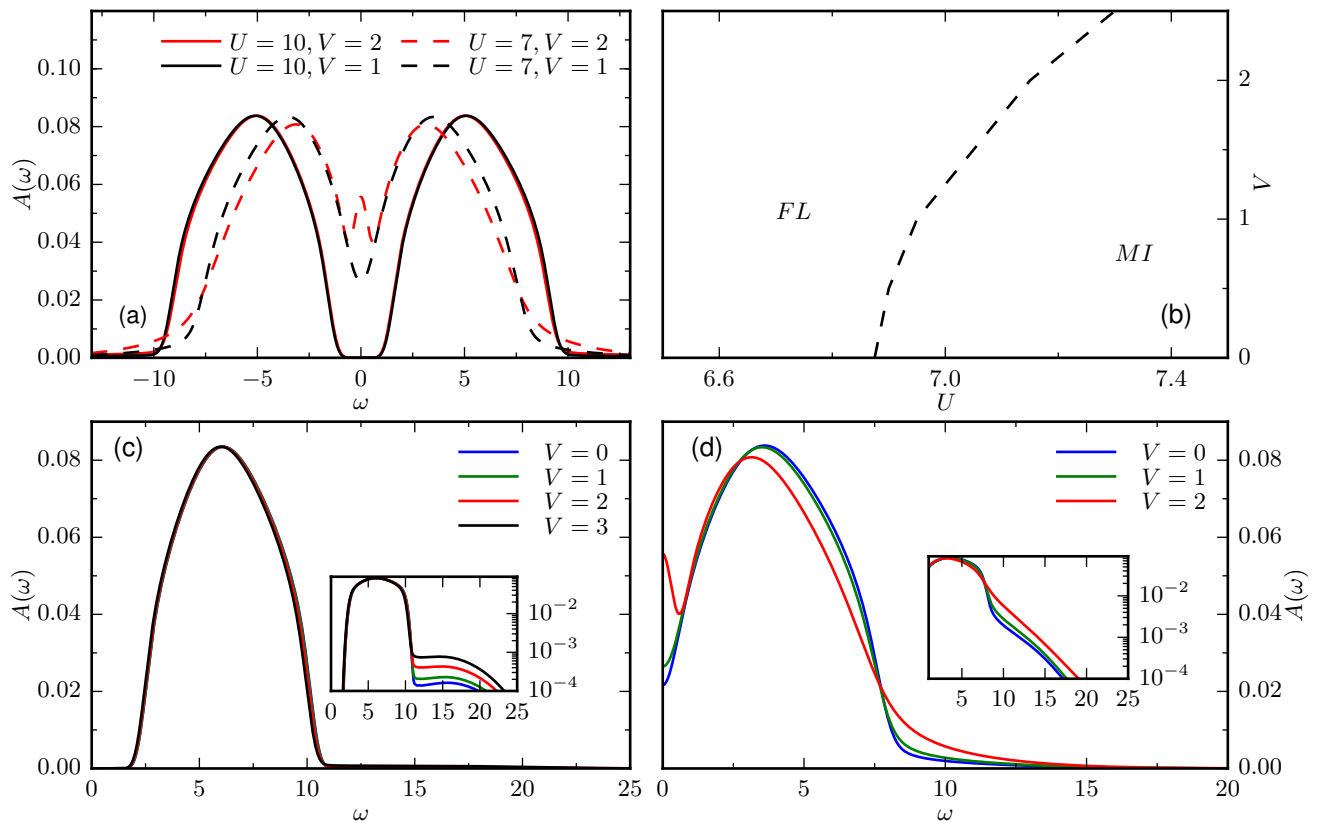
Figure 3. (a) Equilibrium spectral functions for \beta = 20 and indicated values of U and V . (b) Equilibrium phase diagram in the space of U and V at \beta = 20 . The dashed line roughly indicates the metal-insulator crossover defined by the appearance of a quasi-particle peak. (c)-(d) The equilibrium spectral function A(\omega) for U = 12 (c) and U = 7 (d) for indicated values of the nearest neighbor interaction V . The insets show the spectra on a logarithmic scale.
