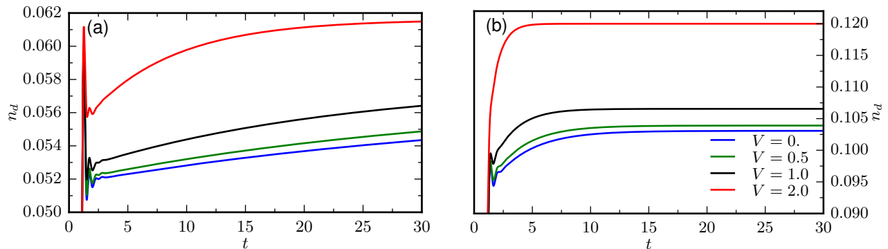
Figure 4. (a),(b) Relaxation dynamics of the double occupancy n_d for different values of V after a pulse with frequency \omega = 10 and pulse amplitude E_0 = 5 . The on-site interaction is U = 10 (a) and U = 7 (b).
