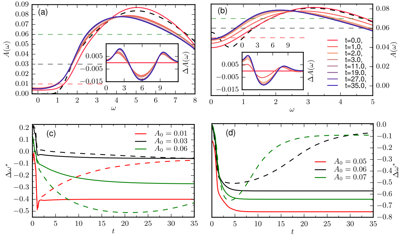
Figure 6. (a,b) Partial Fourier transform of the spectral function A(\omega, t) with insets showing the difference from the initial value A(\omega, t) - A(\omega, t=0) for U = 10, V = 2, E_0 = 5.0 (panel (a)) and U = 7, V = 2, E_0 = 3.5 (panel (b)). The dashed black lines represent the initial equilibrium spectral function. (c,d) Change in the gap size measured by the frequency \omega^* at which the spectral function is equal to some fixed value, A(\omega^*) = A_0 , for U = 10 (c) and U = 7 (d). The dashed lines represent the \omega^* for the same parameters but with coupling to an external bath with \lambda = 1 , see also the discussion in the main text. For U = 7 , there is no intersection for A_0 = 0.05 in the case of coupling to external bath. The corresponding cuts through the spectral function are shown by the dashed lines in panels (a,b).
