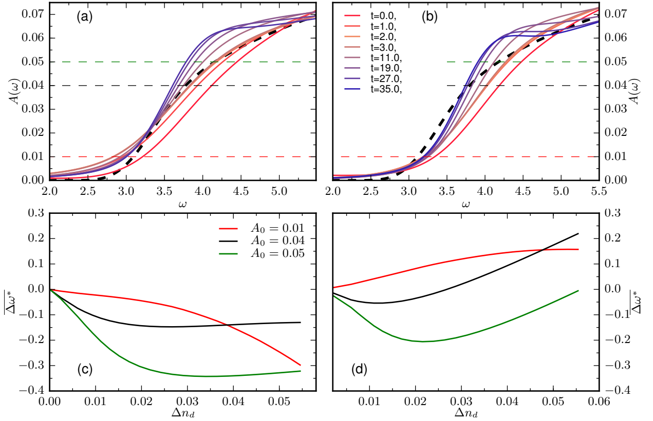
Figure 11. (a,b) Partial Fourier transform of the spectral function A(\omega, t) for U = 14, V = 2, E_0 = 10.0, \omega_0 = 14 (a) and U = 14, V = 0, E_0 = 10.0, \omega = 14 (b) and coupling to a bath with \lambda = 1.0 . The dashed black lines represent the initial equilibrium spectral function. Change in the gap size \omega^* (see discussion in the main text) as a function of the change in the double occupancy \Delta n_d for V = 2 (c) and V = 0 (d).
