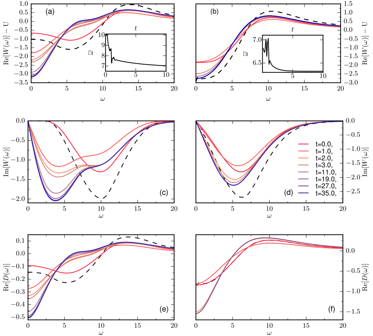
Figure 7. Real (a,b) and imaginary (c,d) part of the partial Fourier transform of the screened interaction \text{Re}[W(t, \omega)] - U for U = 10, E_0 = 5 (left column) and U = 7, E_0 = 3.0 (right column) at fixed V = 2, \omega = 8 . The insets in (a,b) show the evolution of the average boson frequency \bar{\omega}(t) . The black dashed lines represent the screened interaction in the initial equilibrium state. (e,f) Real part of the partial Fourier transform of the regular part of the partially screened on-site interaction \text{Re}[D^{\text{reg}}(t, \omega)] = \text{Re}[\mathcal{U}(t, \omega)] - U for U = 10, E_0 = 5 (e) and U = 7, E_0 = 3.5 (f).
