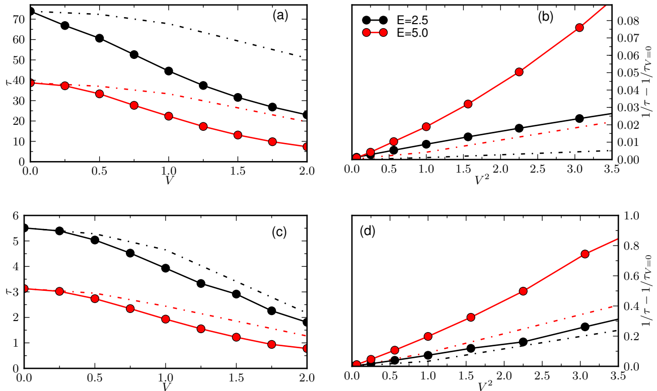
Figure 5. Relaxation time of the double occupancy as a function of nearest neighbour coupling V for U = 10 (a), U = 7 (c), pulse frequency \omega = 10 and pulse amplitudes E_0 = 2.5 and 5 . The dashed lines represent the relaxation time in the Hubbard model with instantaneous interaction U = U(\omega = 0) corresponding to the static interaction in a U - V Hubbard model with a given V (see discussion in the main text). (c,d) Scaling of the difference between the inverse relaxation times at V = 0 and V > 0 with V^2 for the same parameters as in panels (a,c).
