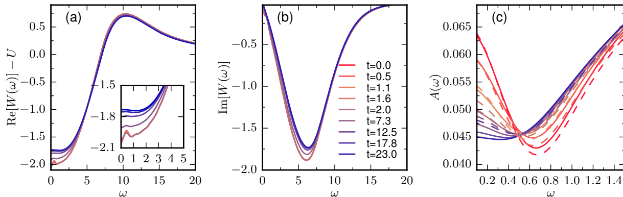
Figure 8. Real (a) and the imaginary (b) part of the partial Fourier transform of the screened interaction W(t, \omega) for U = 6.9 , V = 2 , E = 0.25 , and \omega = 2 . (c) Comparison of the dynamics of the partial Fourier transform of the spectral function A(\omega, t) for the U - V (full lines) model and the Hubbard model (dashed lines) with a correspondingly reduced on-site interaction U = 6.425 .
