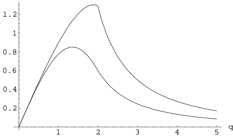
FIG. 9: The functions \frac{3}{8\pi} I(q) [lower curve] and J(q) [upper curve] according to Eqs. (C.1) and (D.1), respectively.
