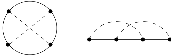
FIG. 4: Feynman diagrams for e_{2x} [11] and \Sigma_{2x} [20].
