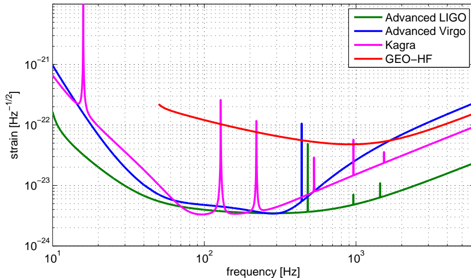
Figure 3. Prediction of the incoherent sum of fundamental noise sources which give a likely best limit to the performance of each of the instruments in the advanced detector network. Noise curves for both Advanced Virgo and KAGRA show a de-tuned signal recycling configuration optimized for sensitivity to neutron star binaries [25, 27, 36], whereas the Advanced LIGO and GEO-HF noise curves are shown with zero de-tuning [37, 38].
